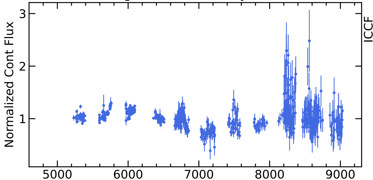
RM728 Light Curves (w/ PyROA model)
