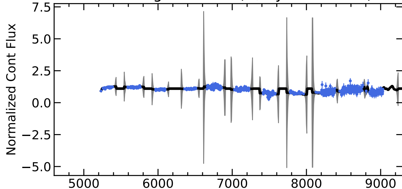
RM729 Light Curves (w/ PyROA model)
