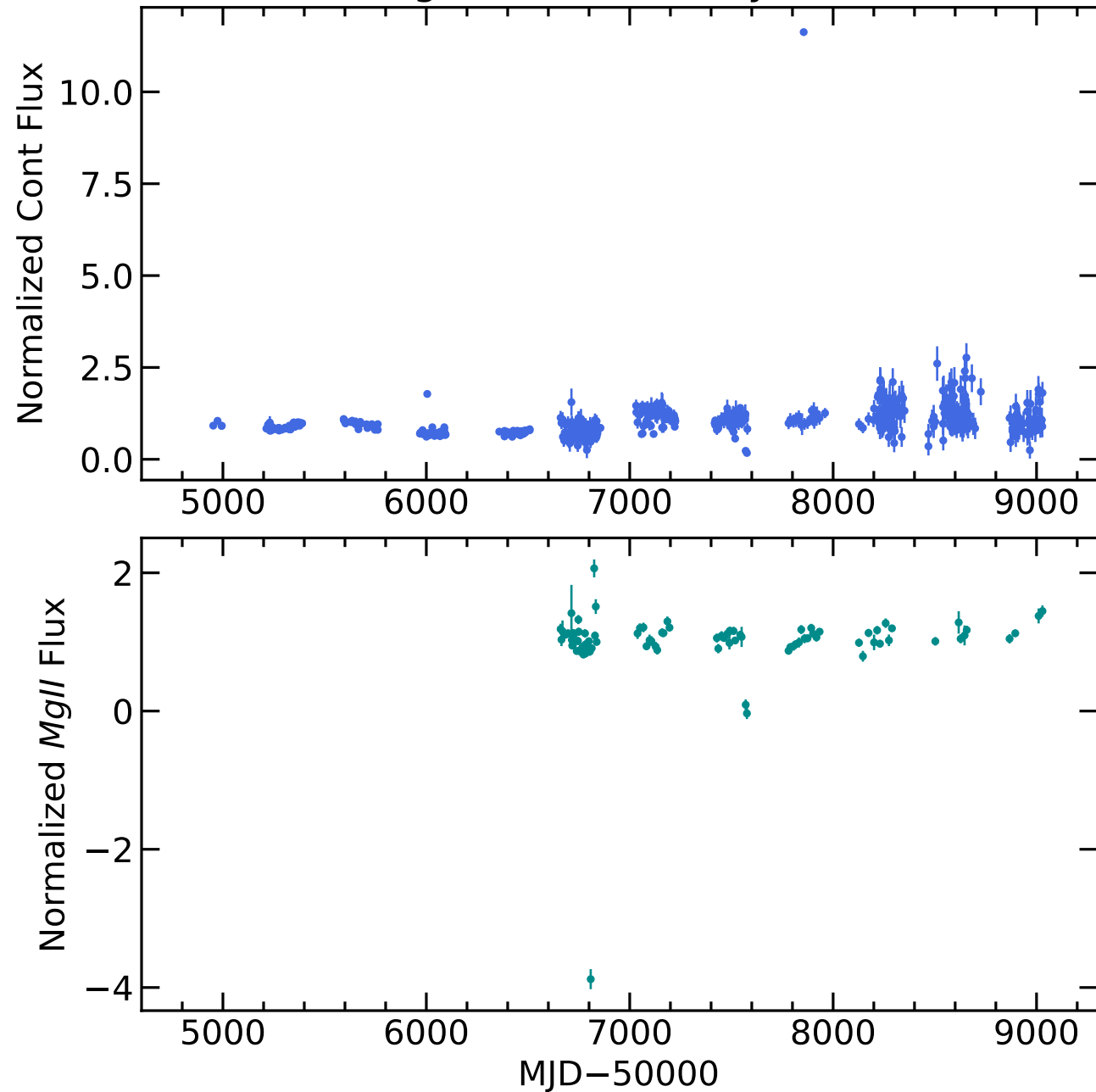
RM732 Light Curves (w/ PyROA model)
