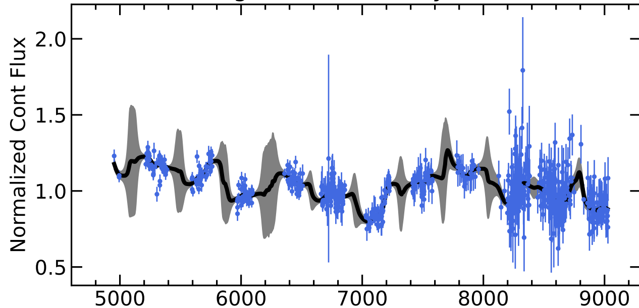
RM733 Light Curves (w/ PyROA model)
