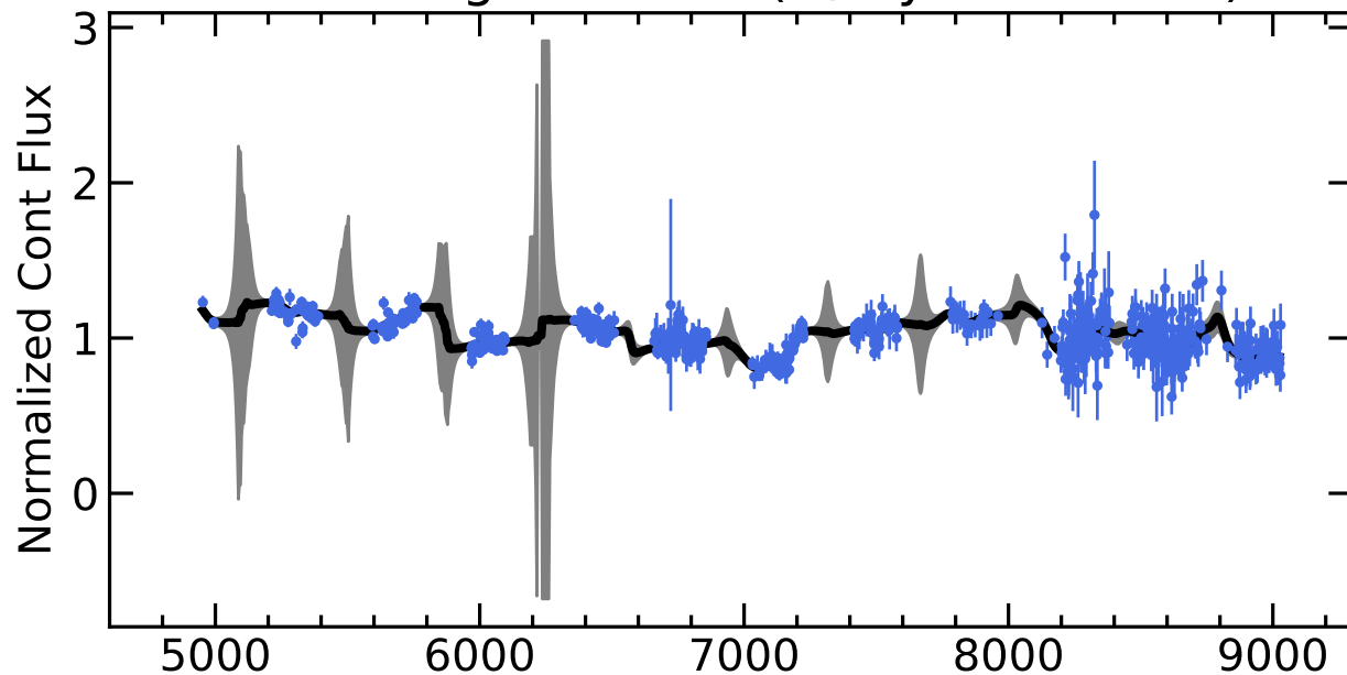
RM733 Light Curves (w/ PyROA model)
