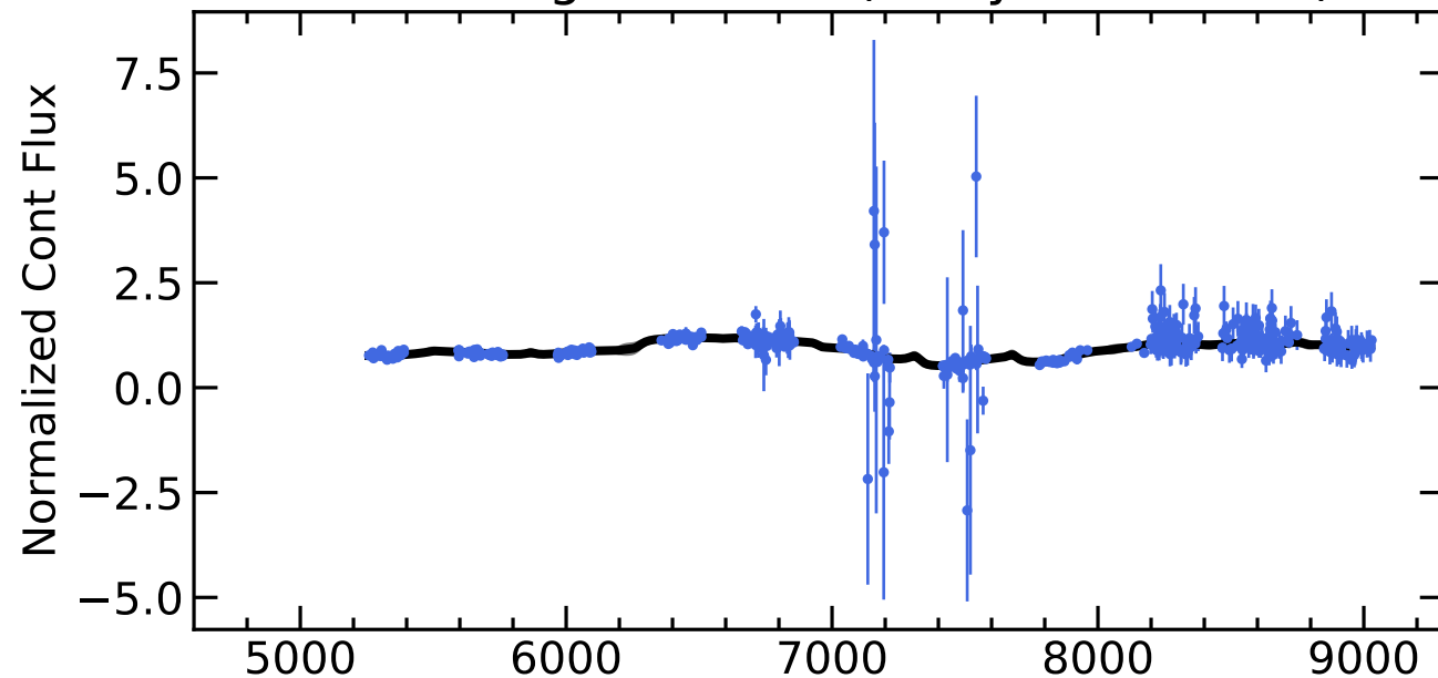
RM734 Light Curves (w/ PyROA model)
