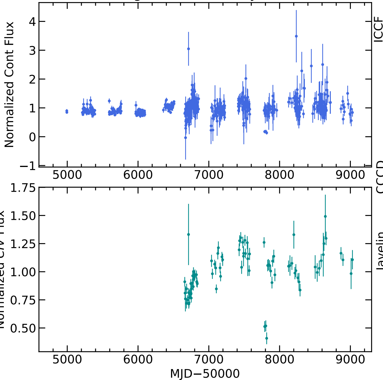
RM735 Light Curves (w/ PyROA model)
