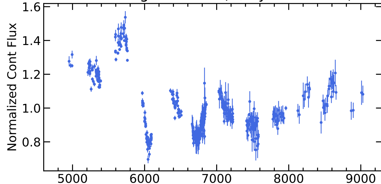
RM736 Light Curves (w/ PyROA model)
