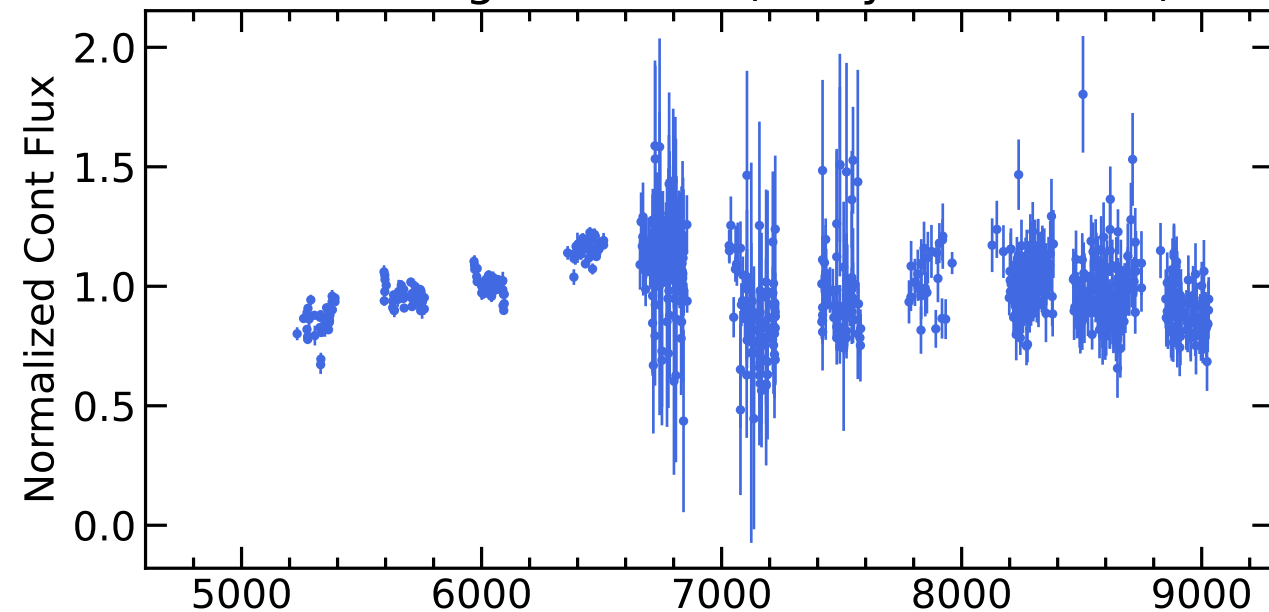
RM738 Light Curves (w/ PyROA model)
