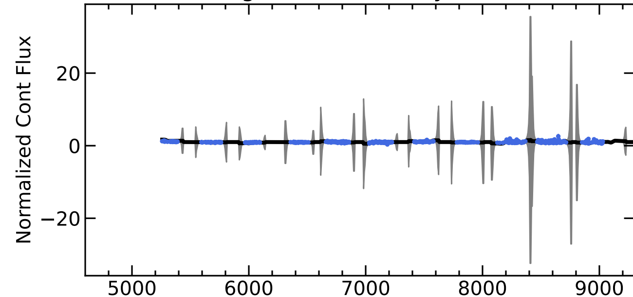
RM739 Light Curves (w/ PyROA model)
