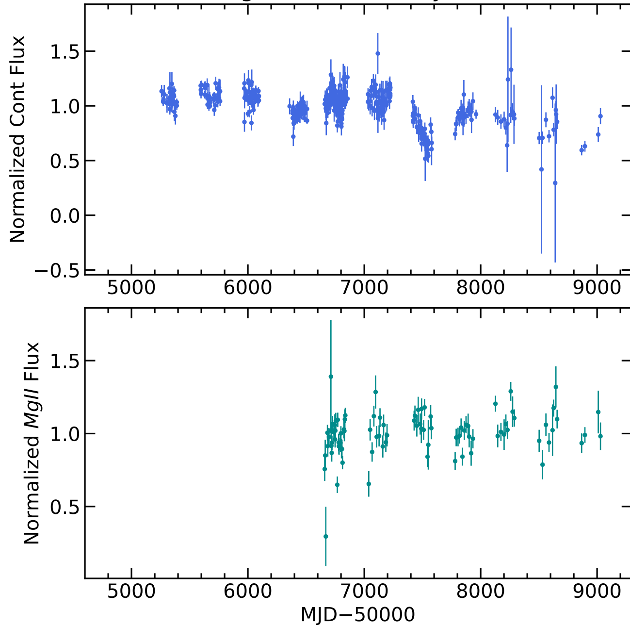
RM741 Light Curves (w/ PyROA model)
