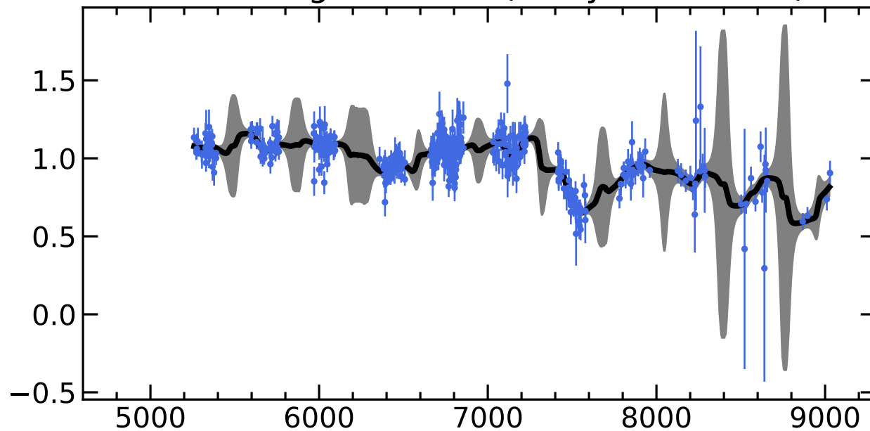
RM741 Light Curves (w/ PyROA model)
