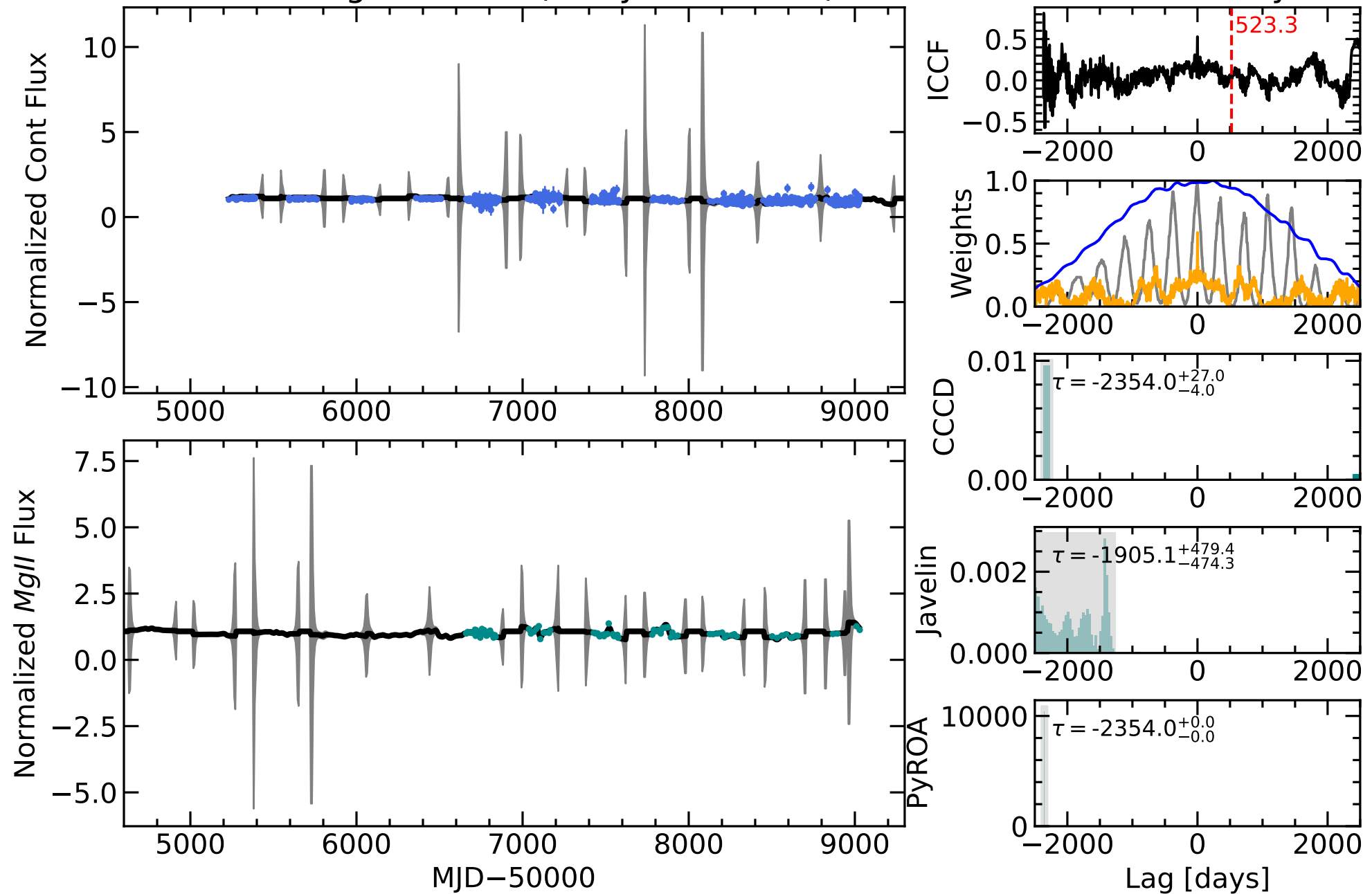
RM743 Light Curves (w/ PyROA model)
