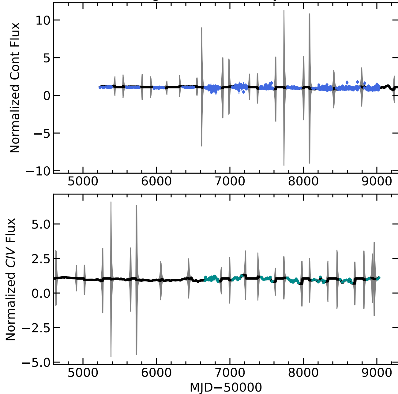
RM743 Light Curves (w/ PyROA model)
