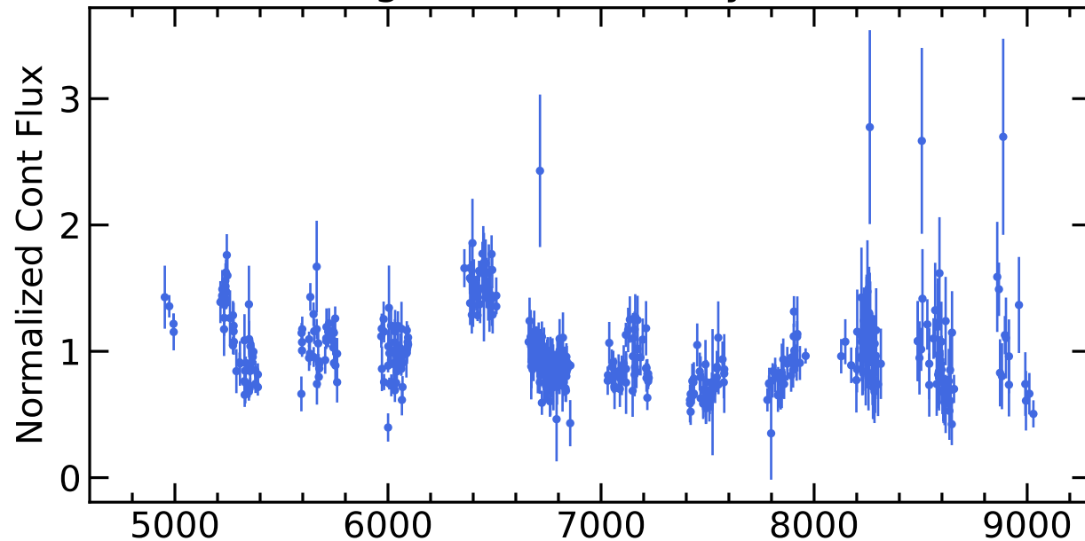
RM744 Light Curves (w/ PyROA model)
