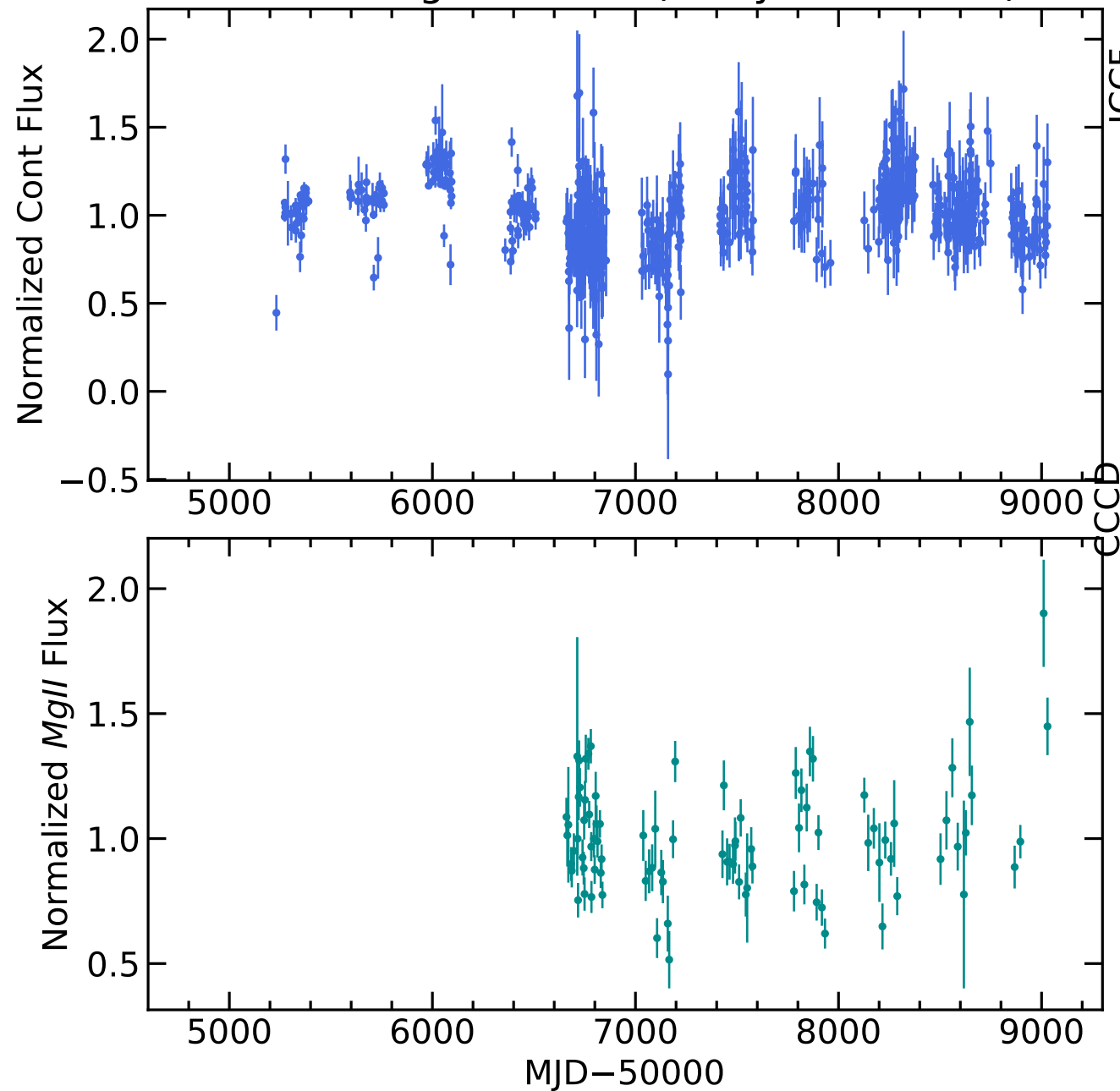
RM745 Light Curves (w/ PyROA model)
