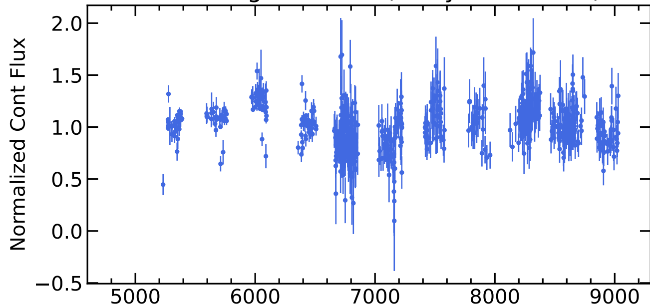
RM745 Light Curves (w/ PyROA model)
