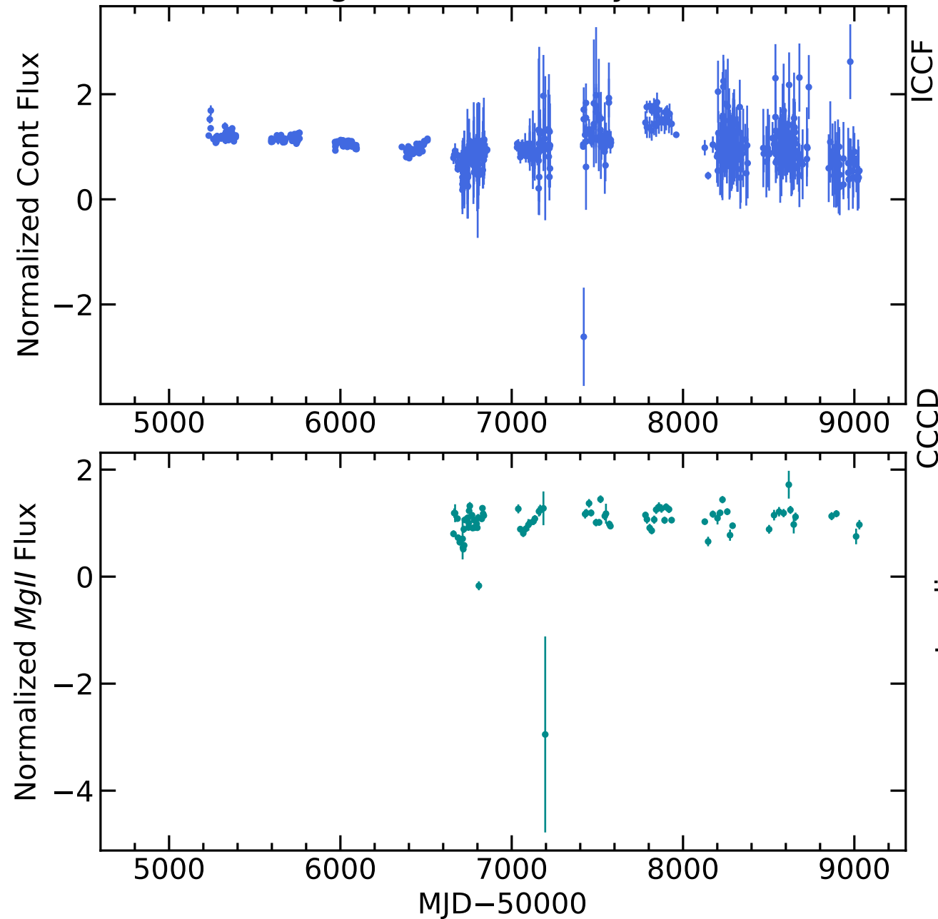
RM747 Light Curves (w/ PyROA model)
