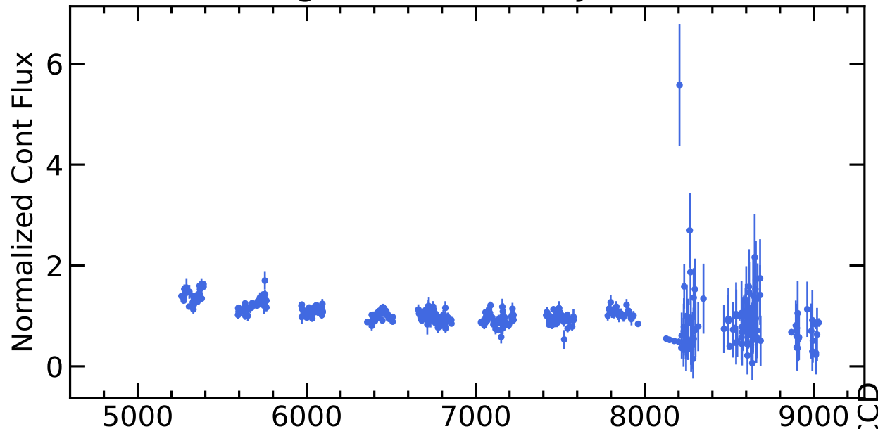
RM748 Light Curves (w/ PyROA model)
