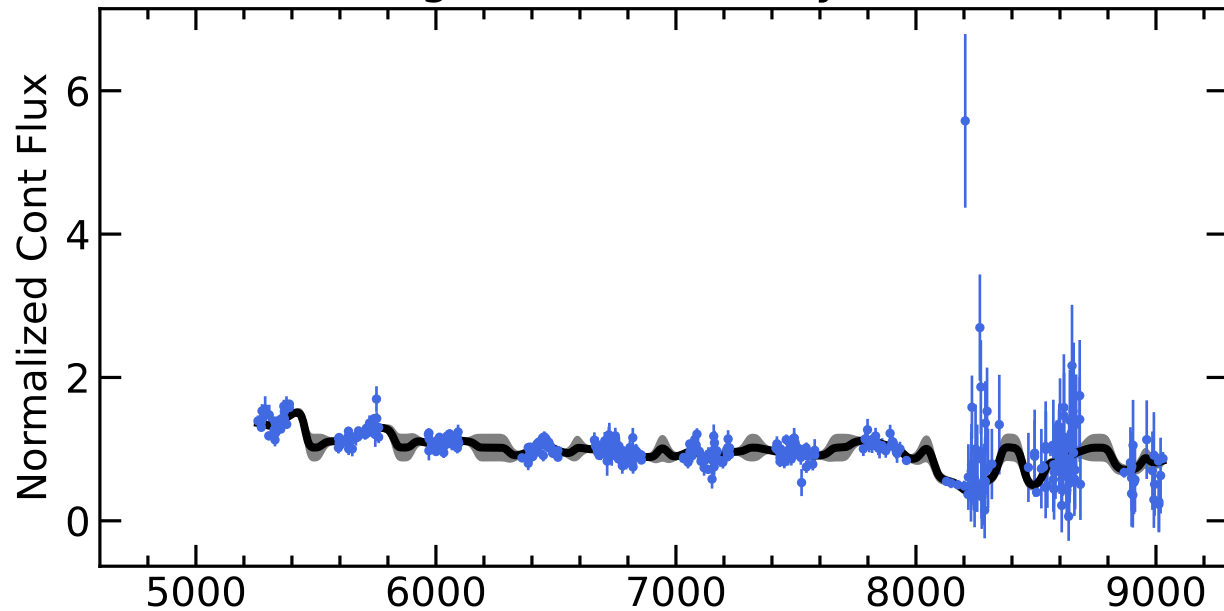
RM748 Light Curves (w/ PyROA model)
