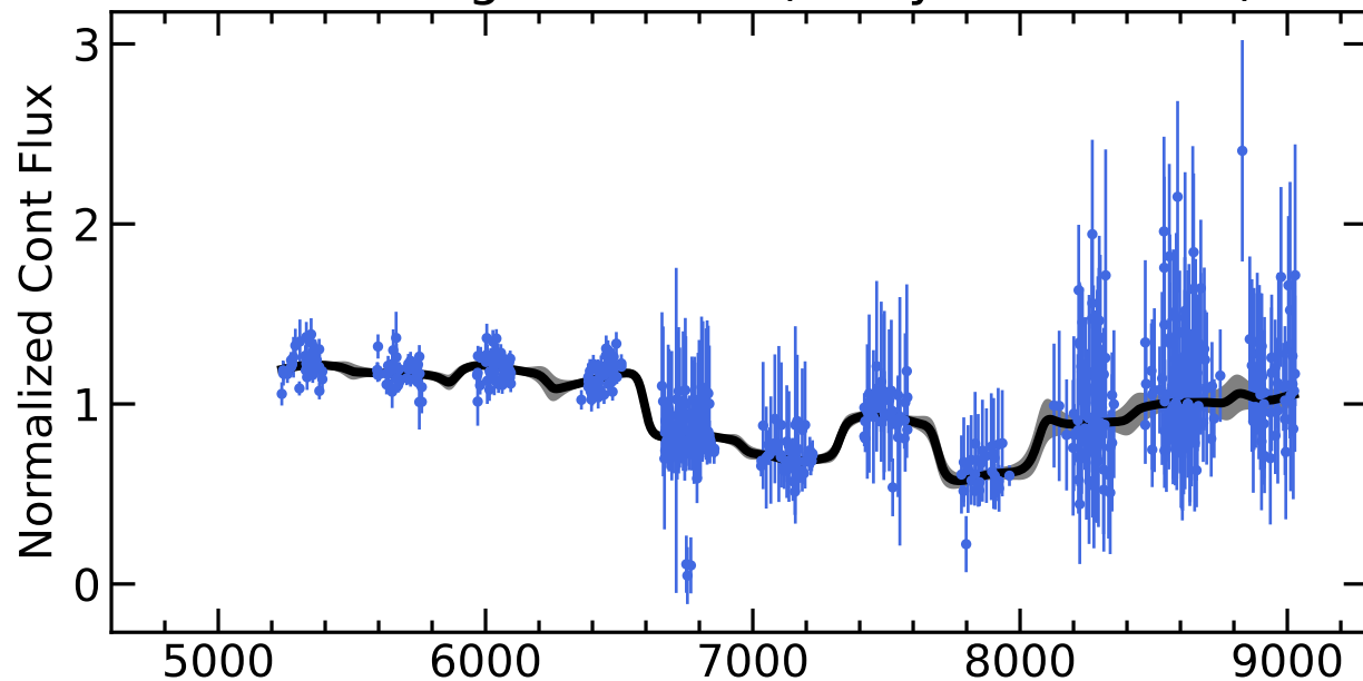
RM749 Light Curves (w/ PyROA model)
