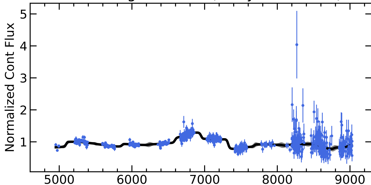
RM751 Light Curves (w/ PyROA model)
