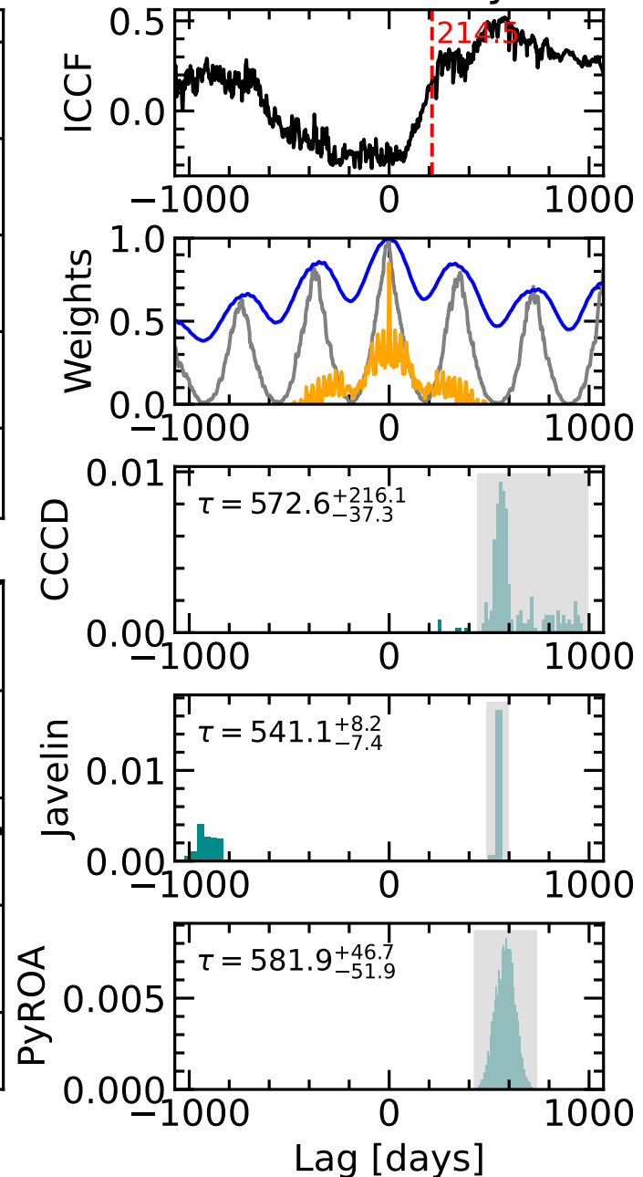
Time Delay
