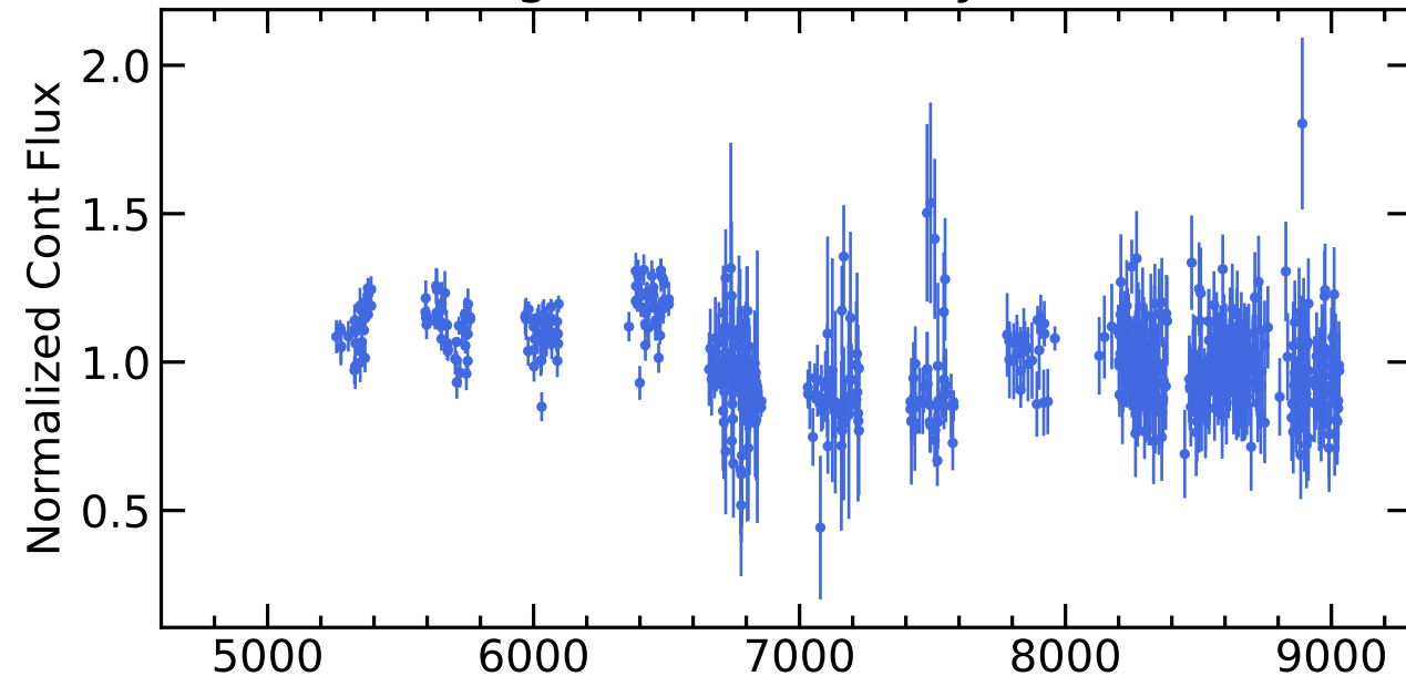
RM753 Light Curves (w/ PyROA model)
