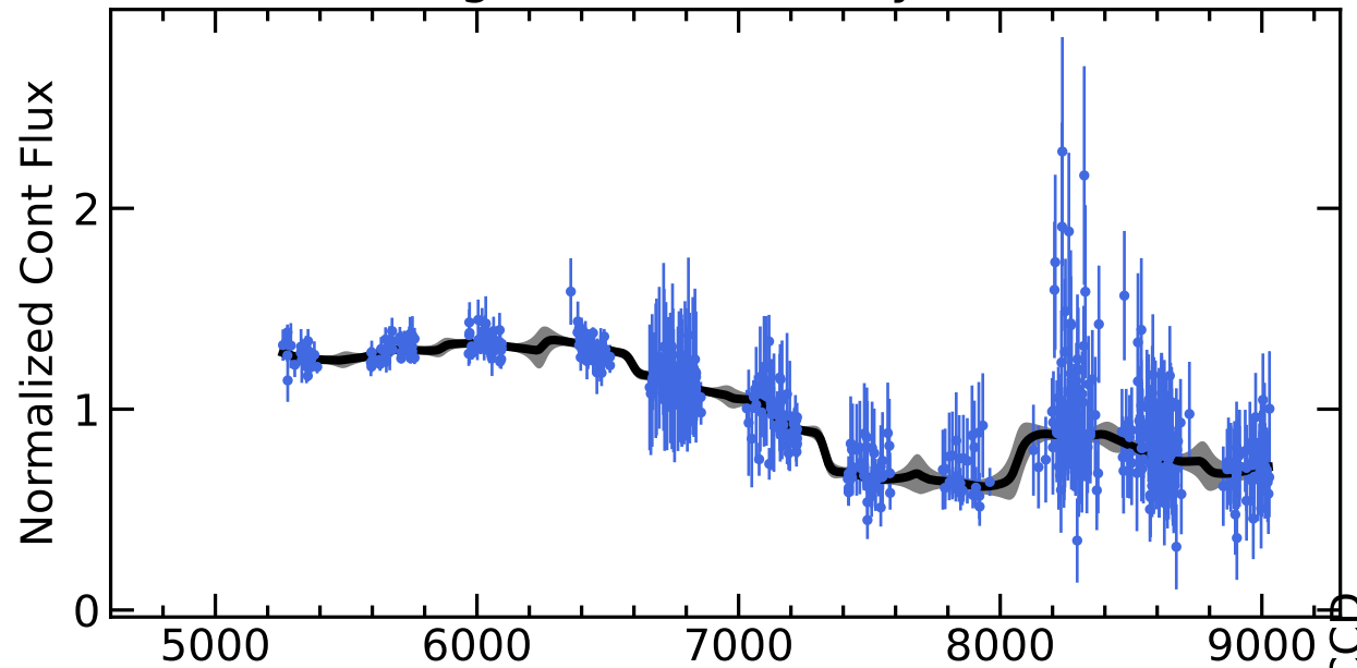
RM754 Light Curves (w/ PyROA model)
