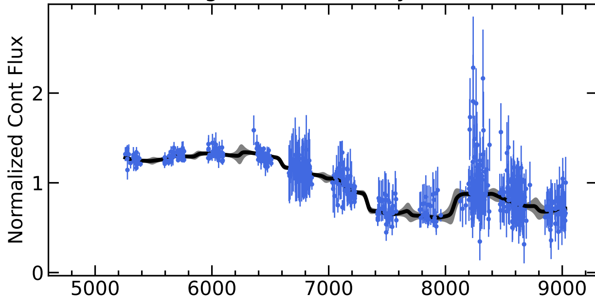
RM754 Light Curves (w/ PyROA model)
