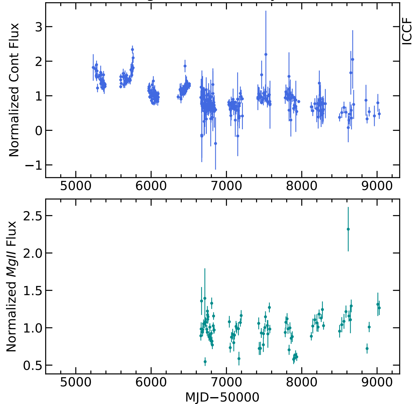
RM755 Light Curves (w/ PyROA model)
