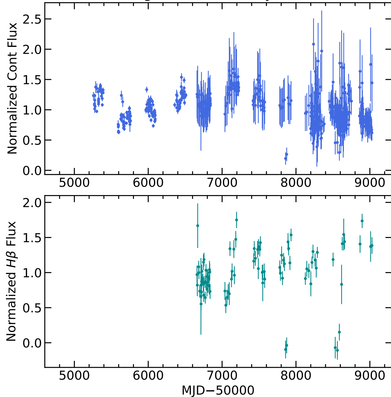
RM756 Light Curves (w/ PyROA model)
