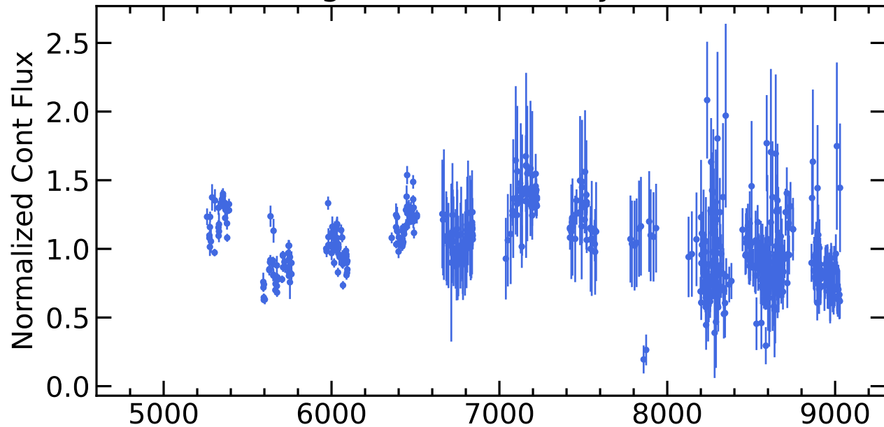
RM756 Light Curves (w/ PyROA model)
