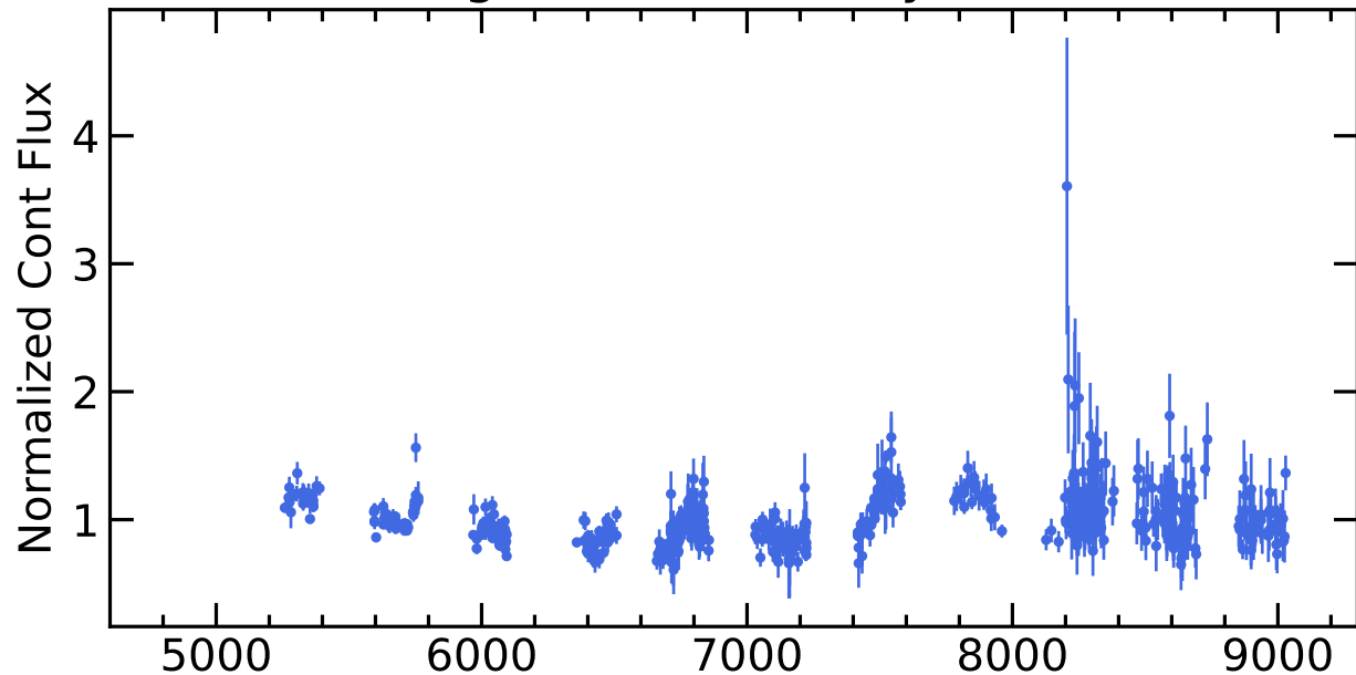
RM757 Light Curves (w/ PyROA model)
