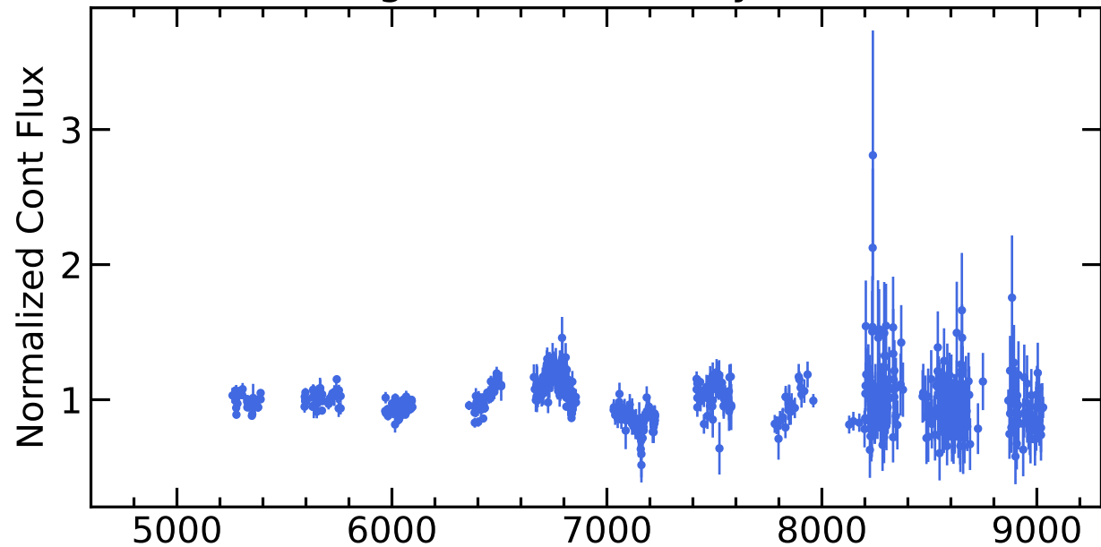
RM758 Light Curves (w/ PyROA model)
