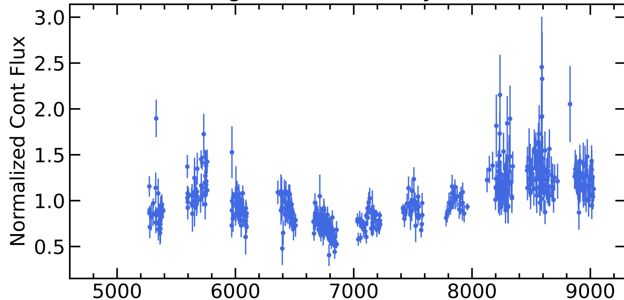
RM759 Light Curves (w/ PyROA model)
