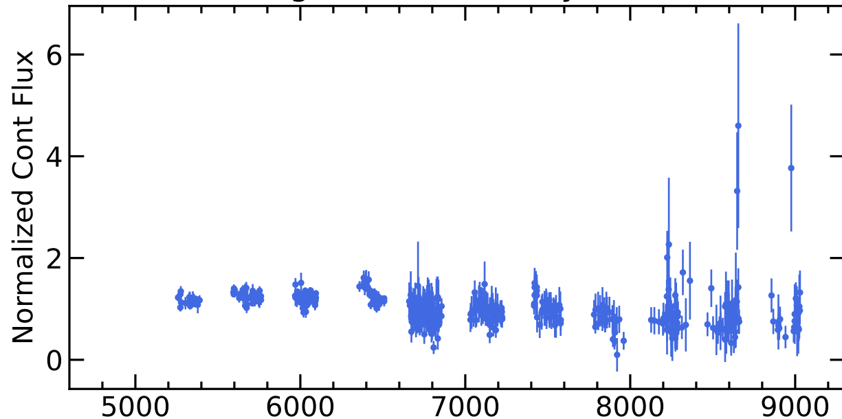
RM760 Light Curves (w/ PyROA model)
