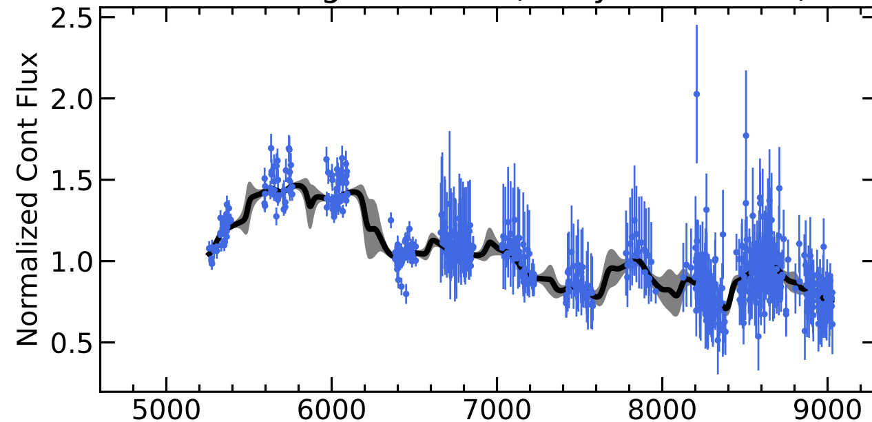
RM761 Light Curves (w/ PyROA model)
