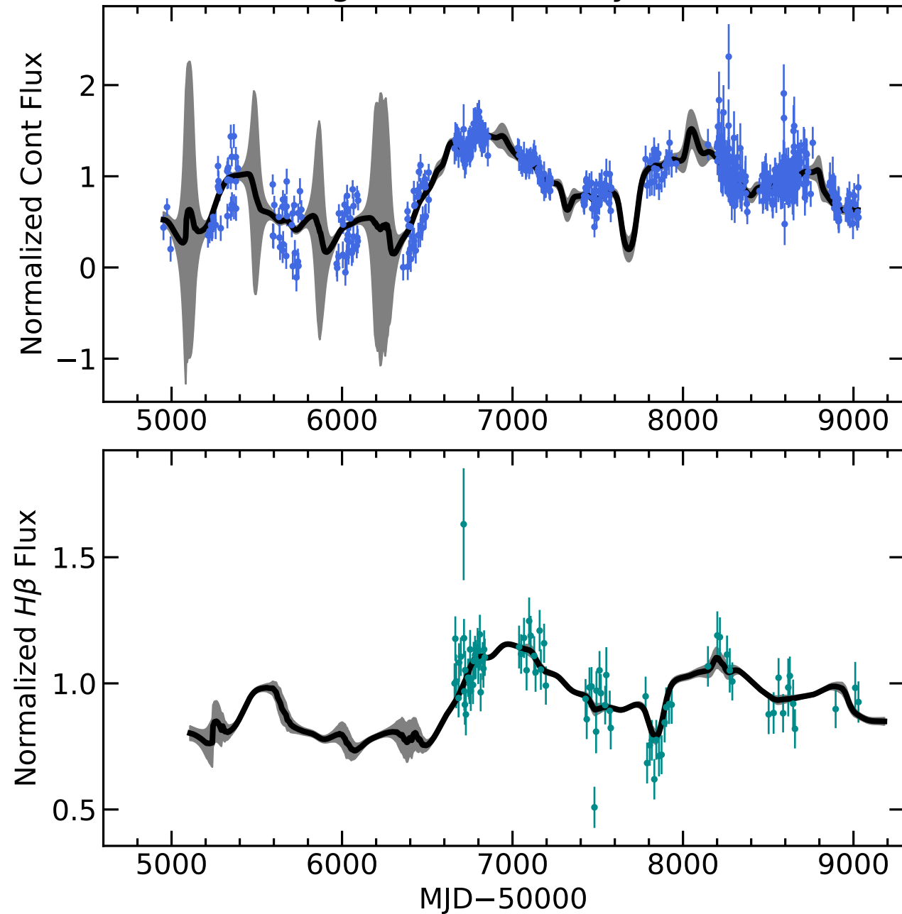
RM762 Light Curves (w/ PyROA model)
