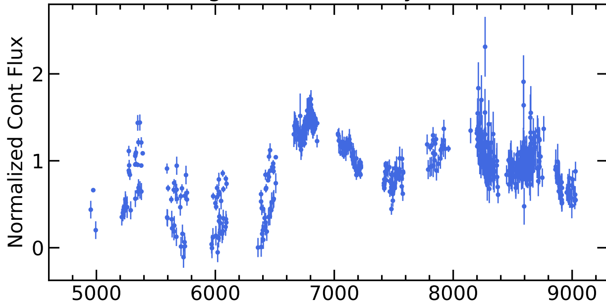
RM762 Light Curves (w/ PyROA model)
