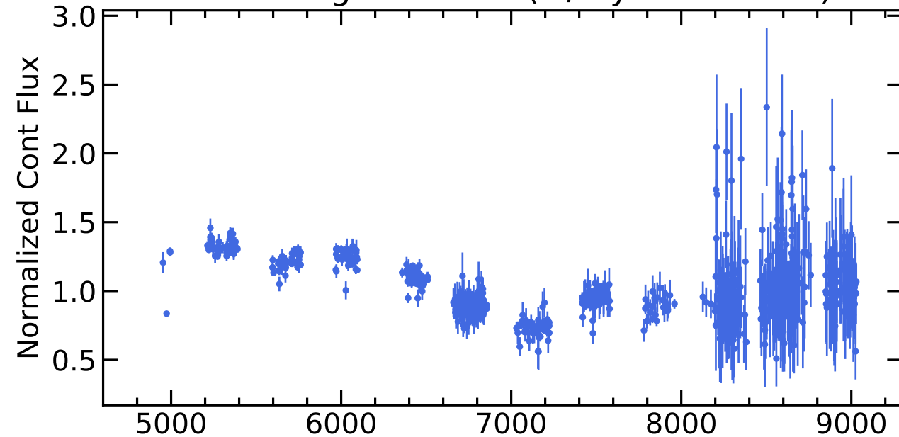
RM763 Light Curves (w/ PyROA model)
