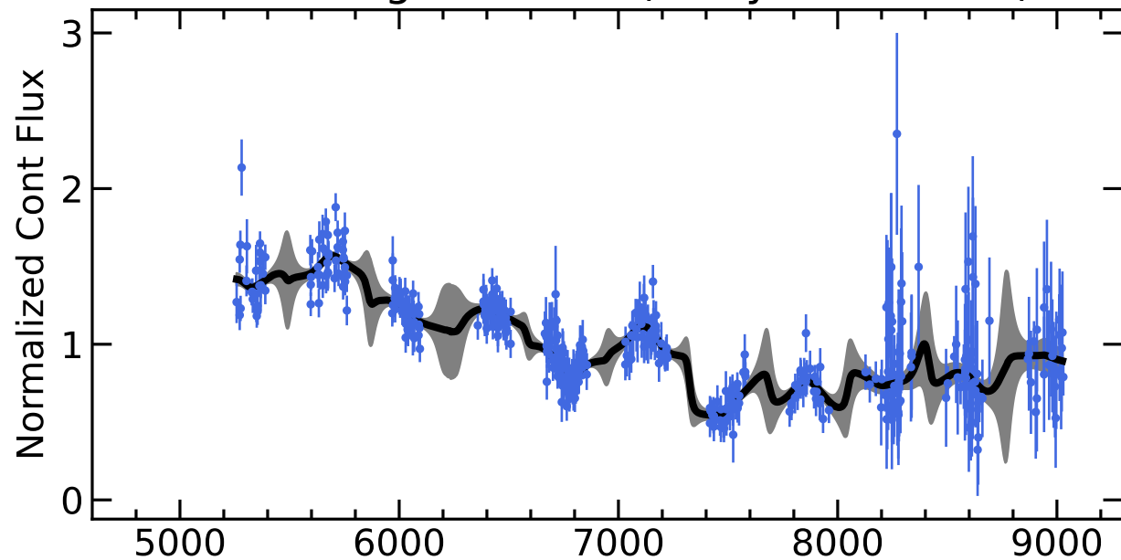
RM764 Light Curves (w/ PyROA model)
