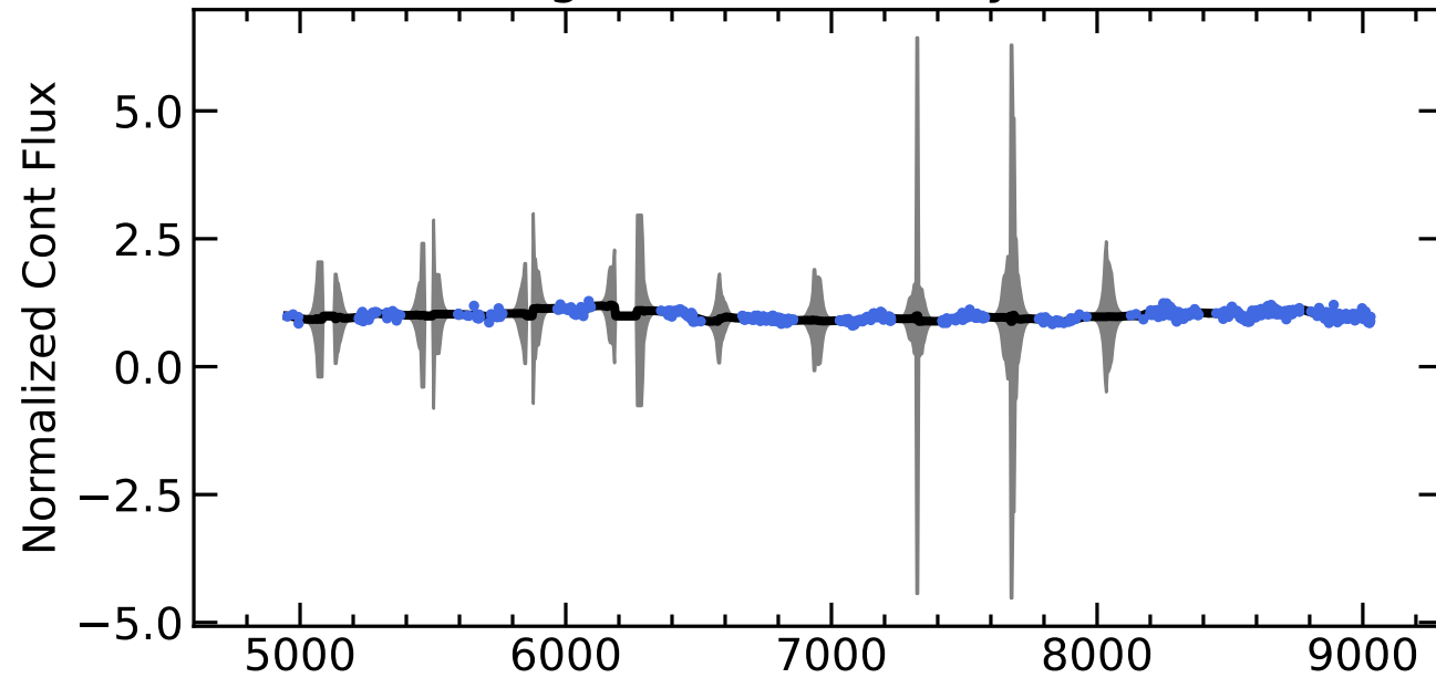
RM766 Light Curves (w/ PyROA model)
