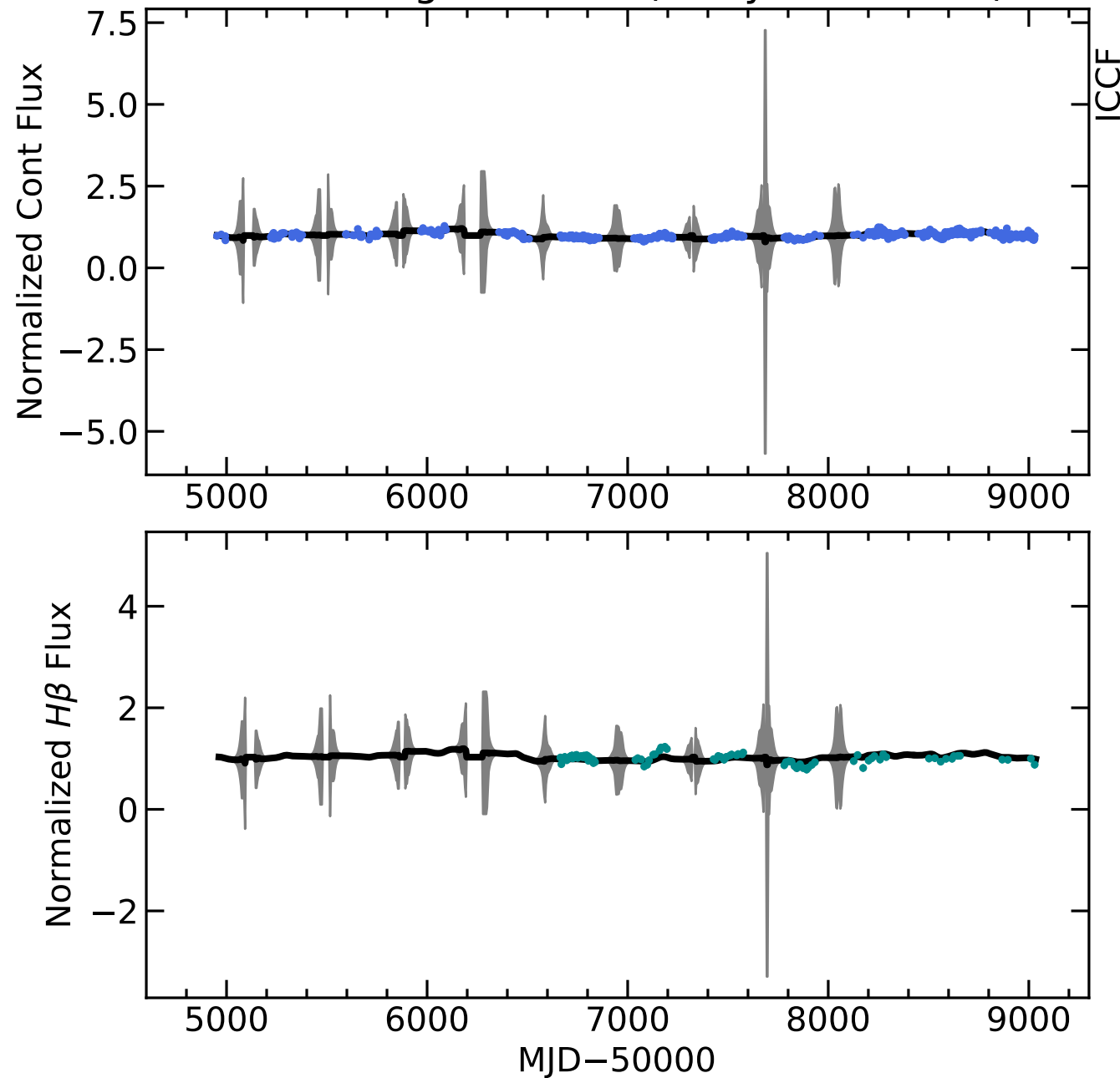
RM766 Light Curves (w/ PyROA model)
