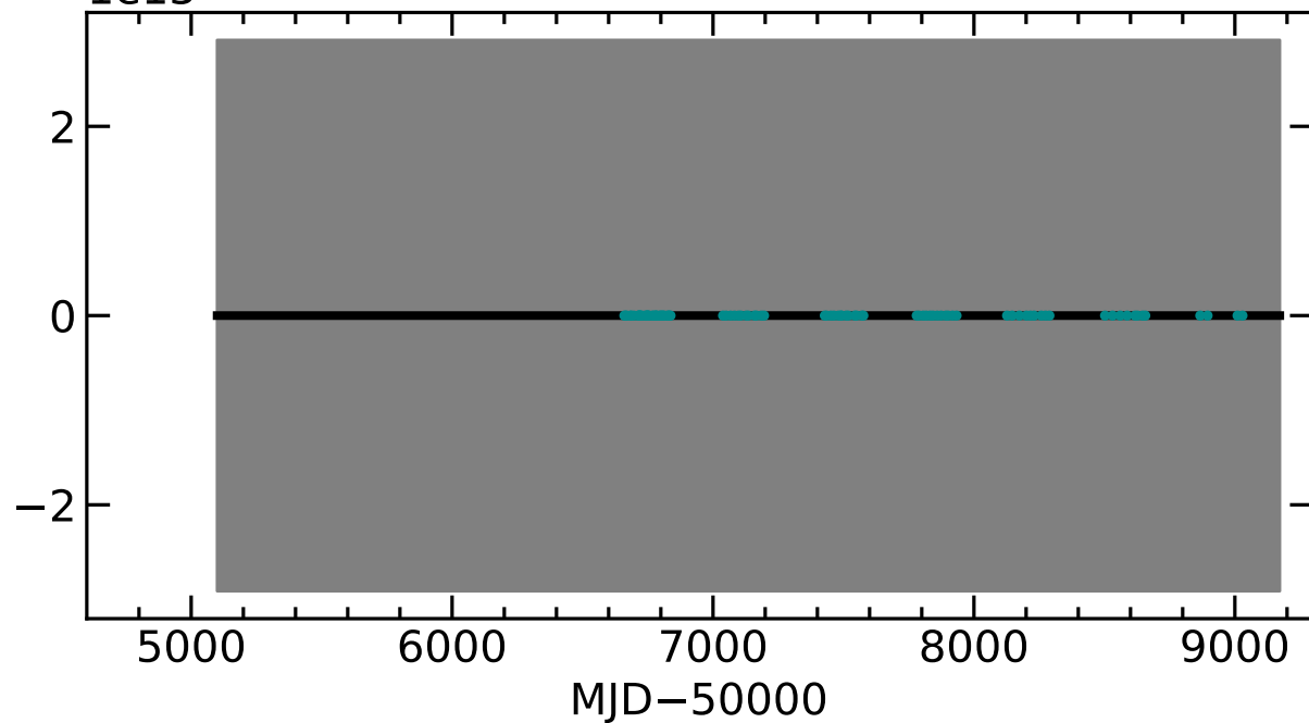
Normalized H\beta Flux
