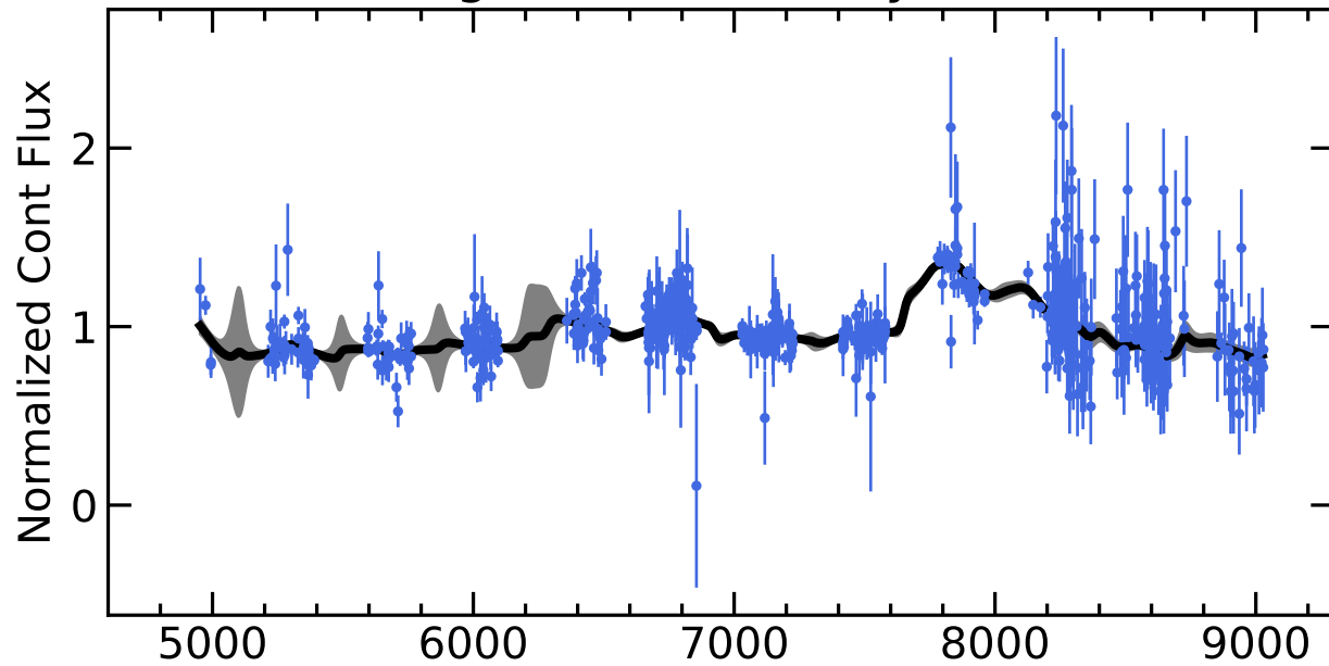
RM767 Light Curves (w/ PyROA model)
