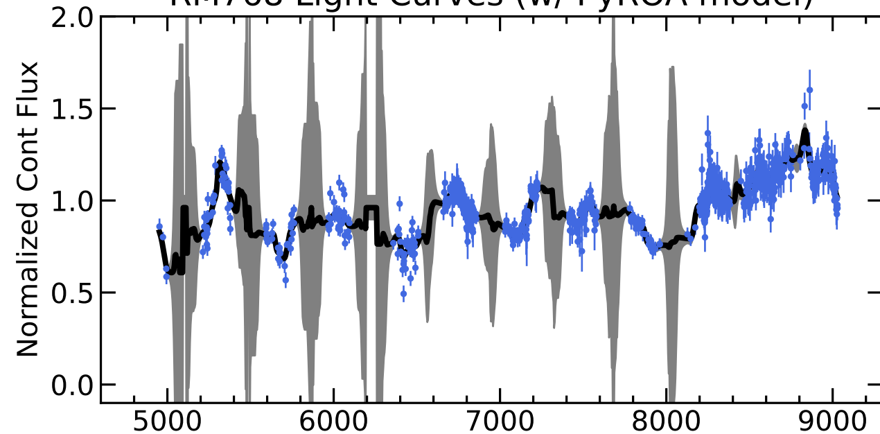
RM768 Light Curves (w/ PyROA model)
