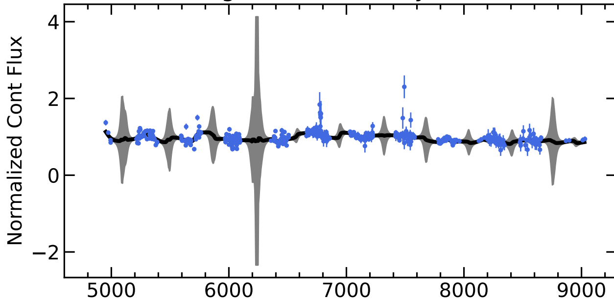
RM769 Light Curves (w/ PyROA model)
