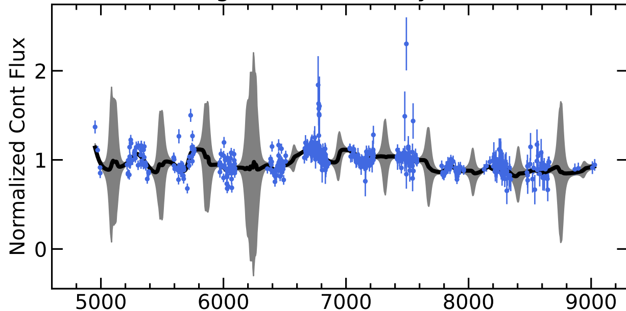
RM769 Light Curves (w/ PyROA model)
