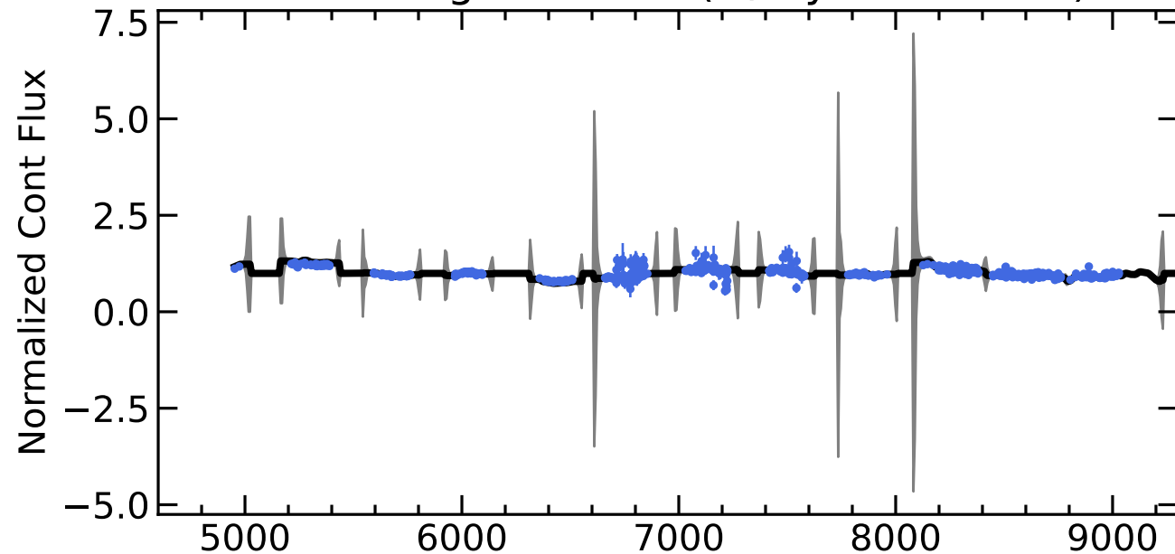
RM771 Light Curves (w/ PyROA model)
