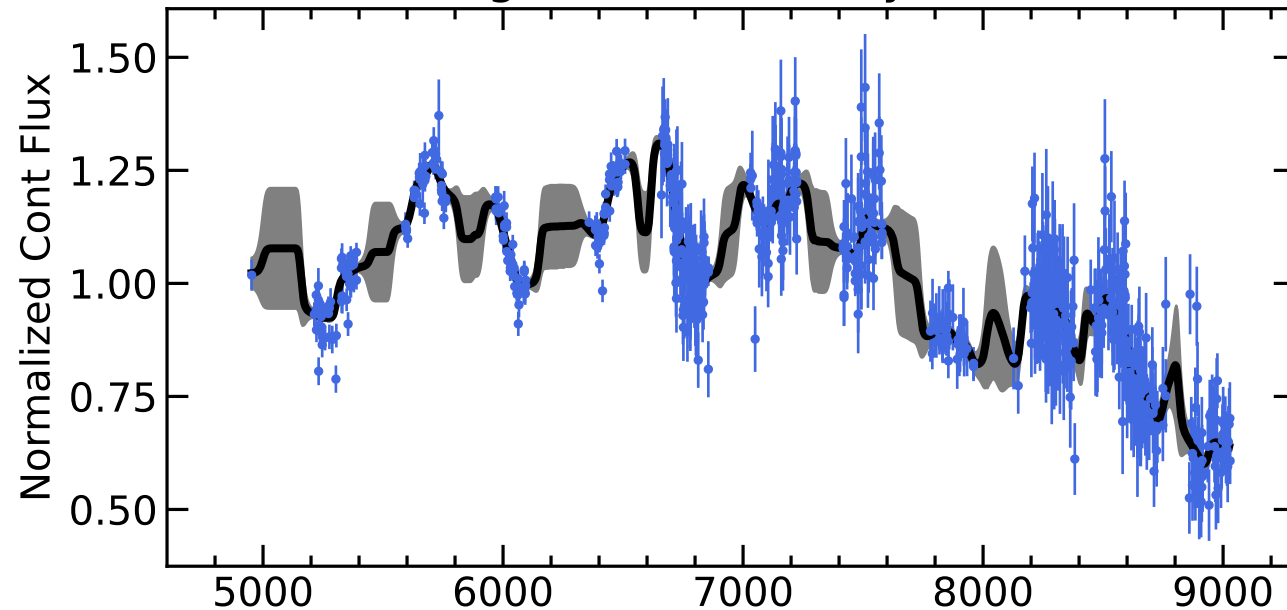
RM773 Light Curves (w/ PyROA model)
