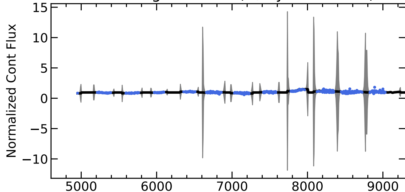
RM774 Light Curves (w/ PyROA model)
