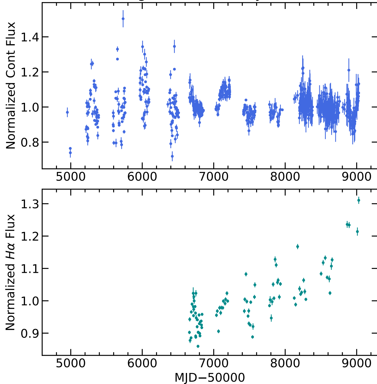
RM775 Light Curves (w/ PyROA model)
