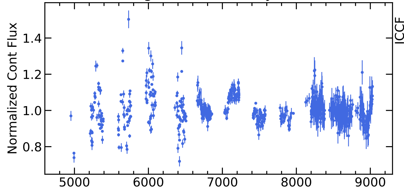
RM775 Light Curves (w/ PyROA model)
