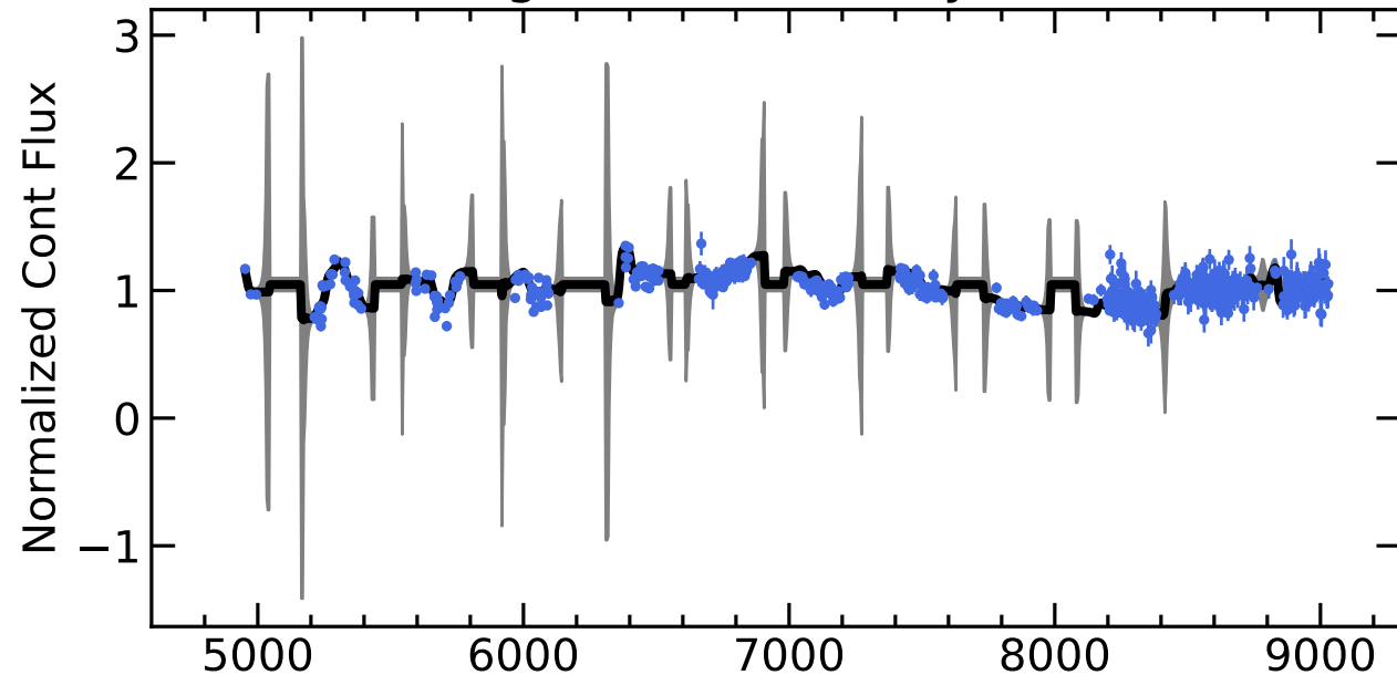
RM776 Light Curves (w/ PyROA model)
