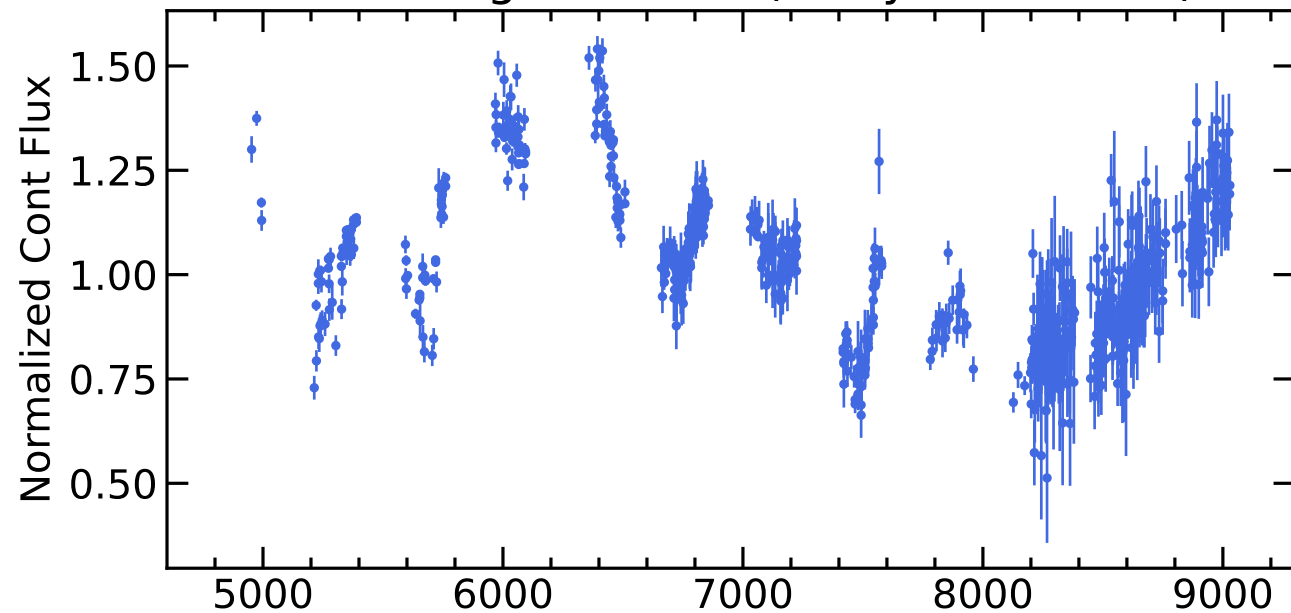
RM778 Light Curves (w/ PyROA model)
