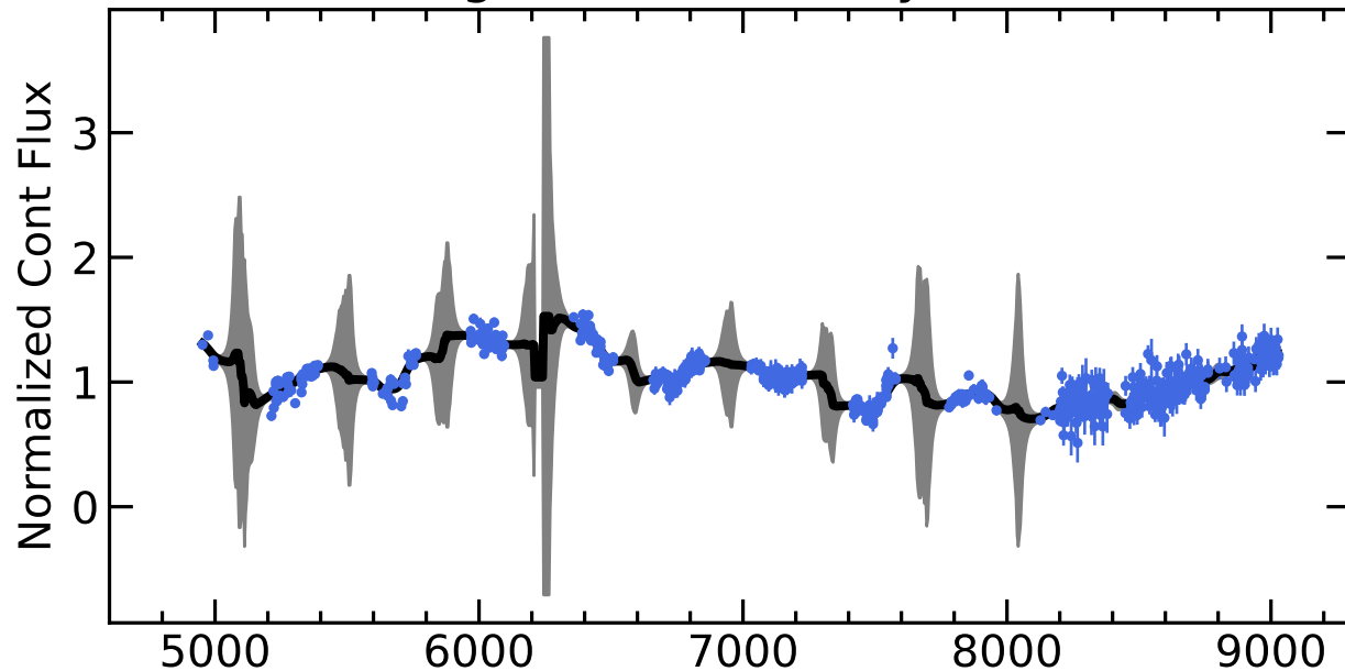
RM778 Light Curves (w/ PyROA model)
