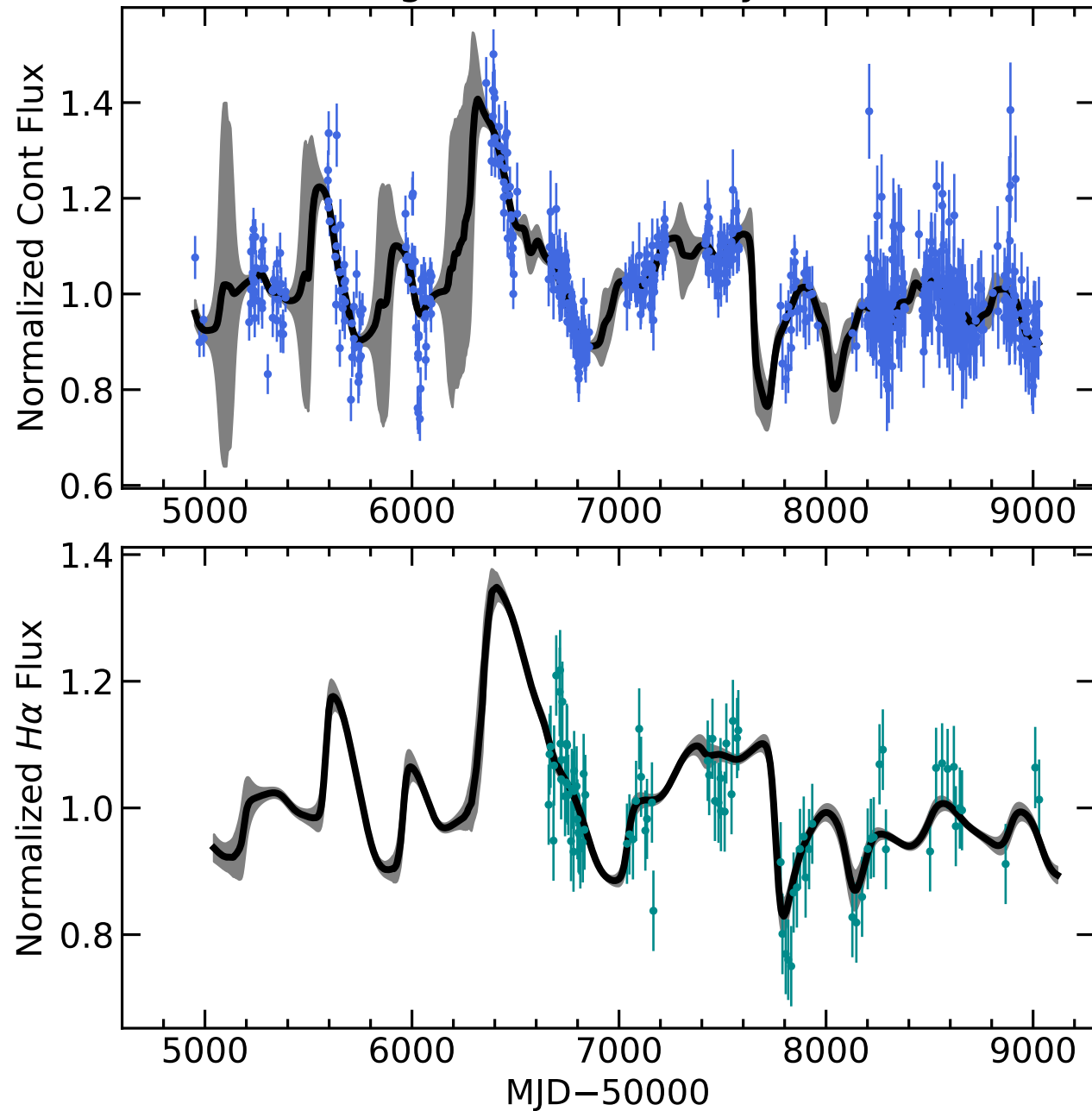
RM779 Light Curves (w/ PyROA model)
