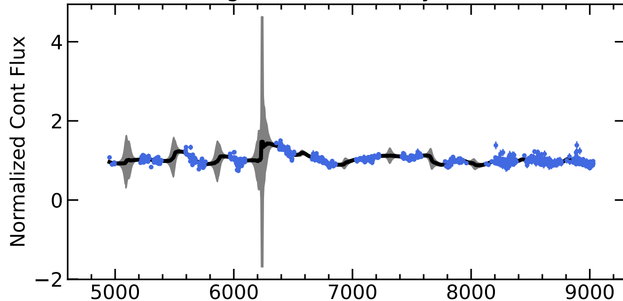
RM779 Light Curves (w/ PyROA model)
