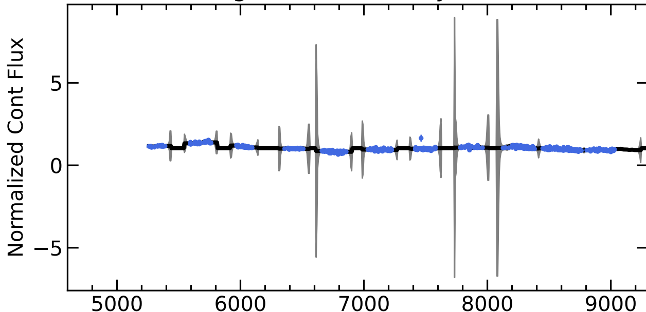
RM780 Light Curves (w/ PyROA model)
