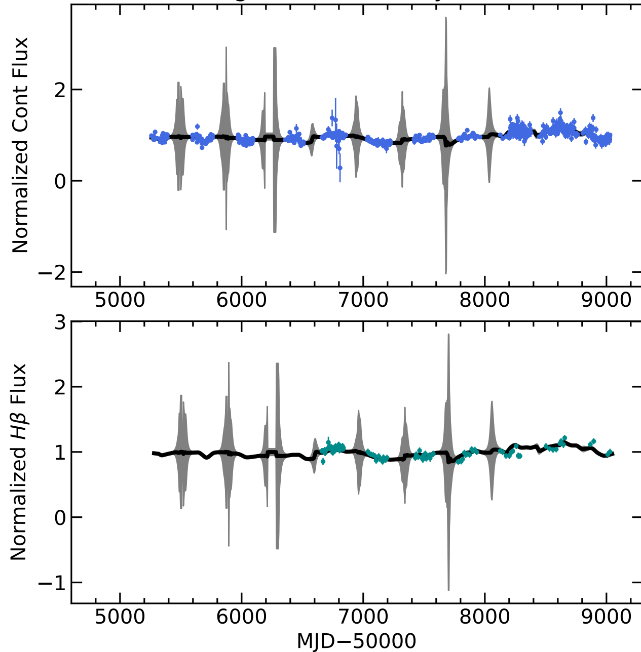
RM781 Light Curves (w/ PyROA model)
