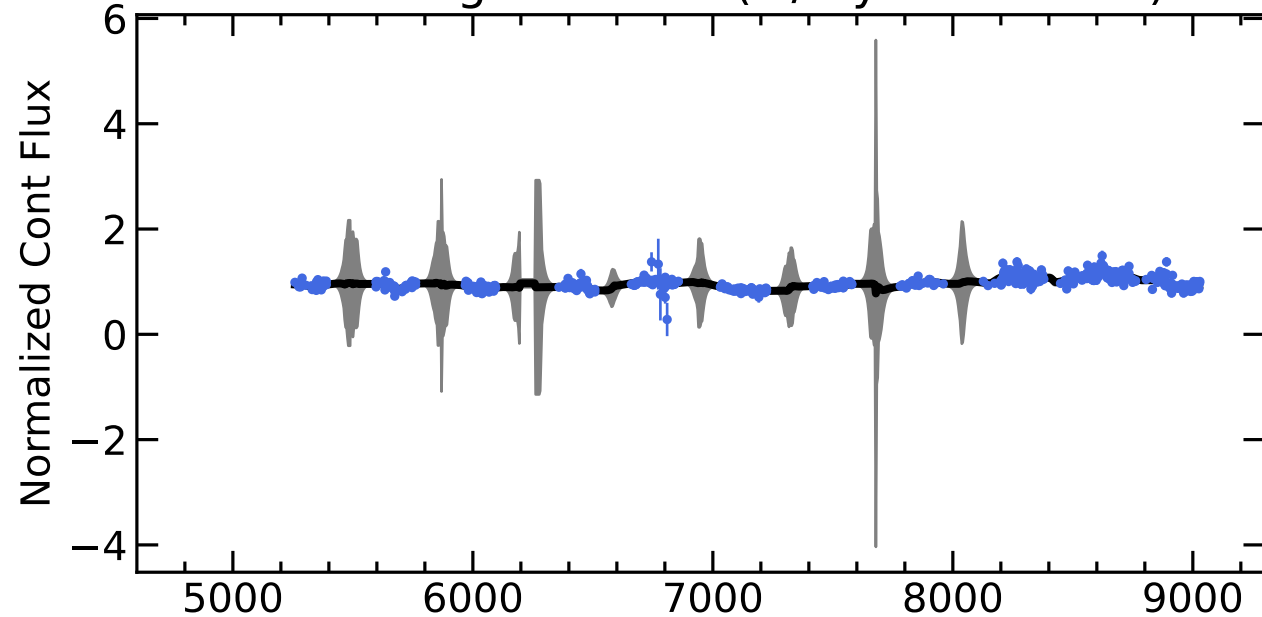
RM781 Light Curves (w/ PyROA model)
