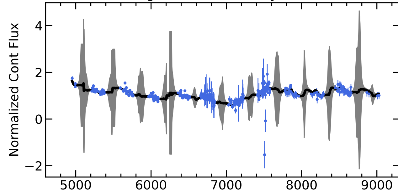
RM782 Light Curves (w/ PyROA model)
