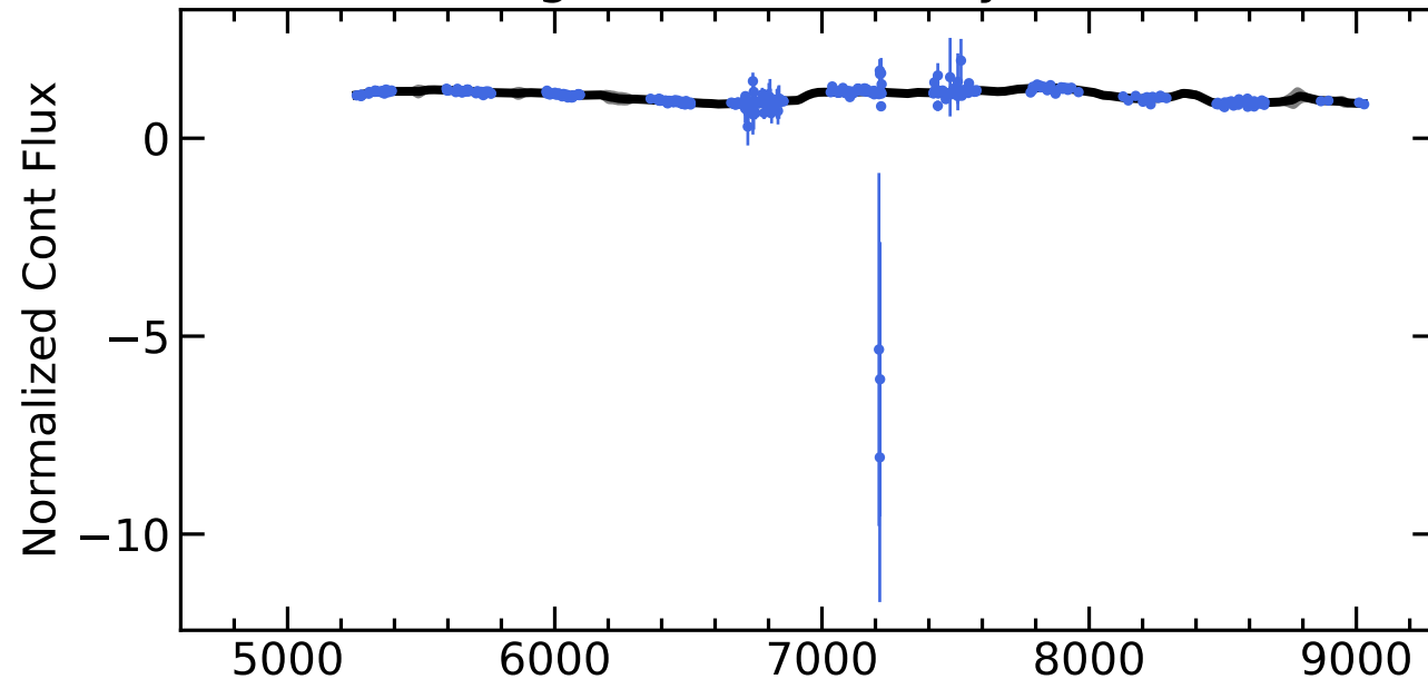
RM783 Light Curves (w/ PyROA model)
