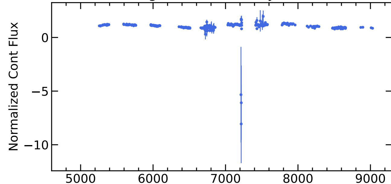
RM783 Light Curves (w/ PyROA model)
