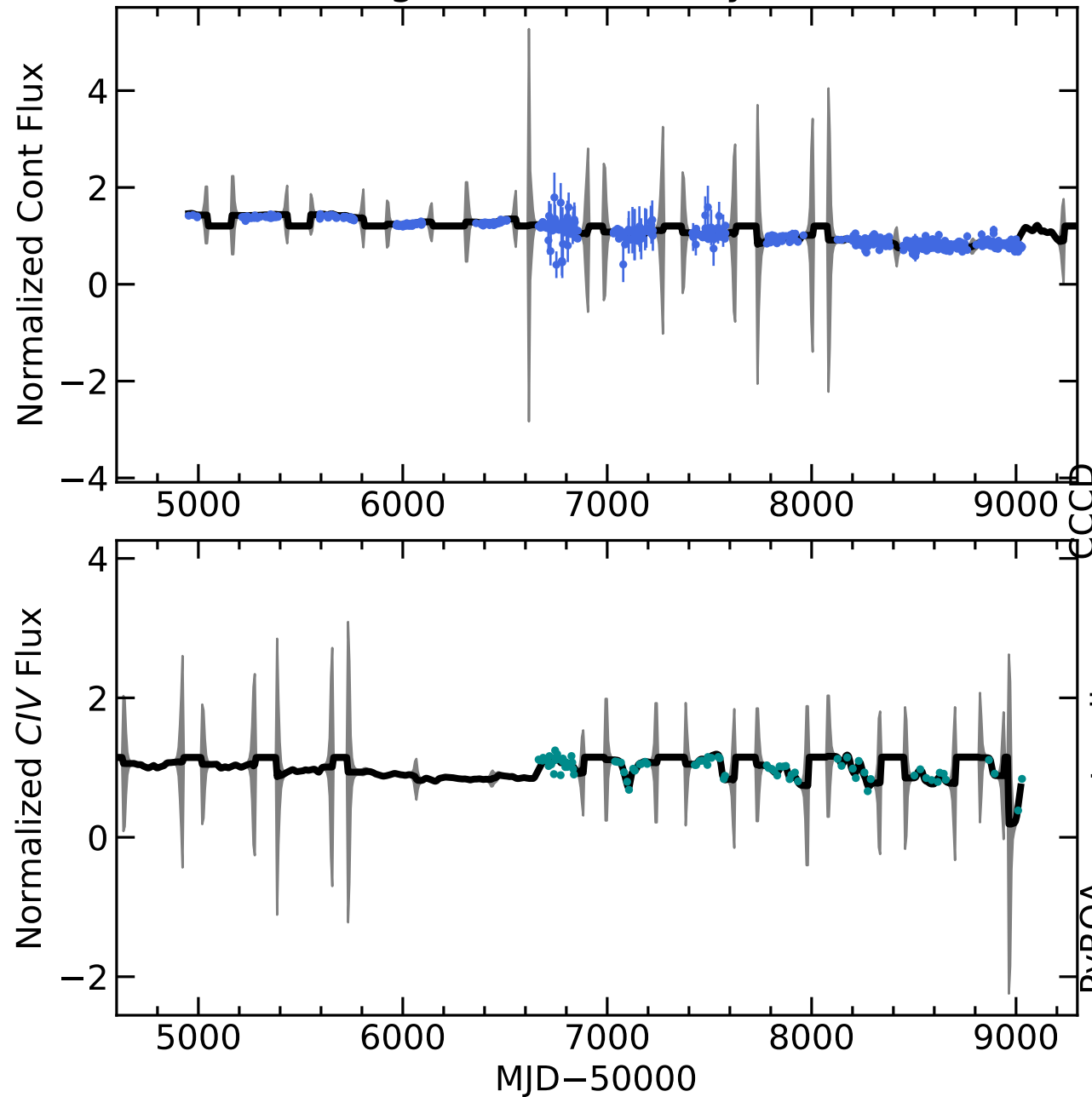
RM784 Light Curves (w/ PyROA model)
