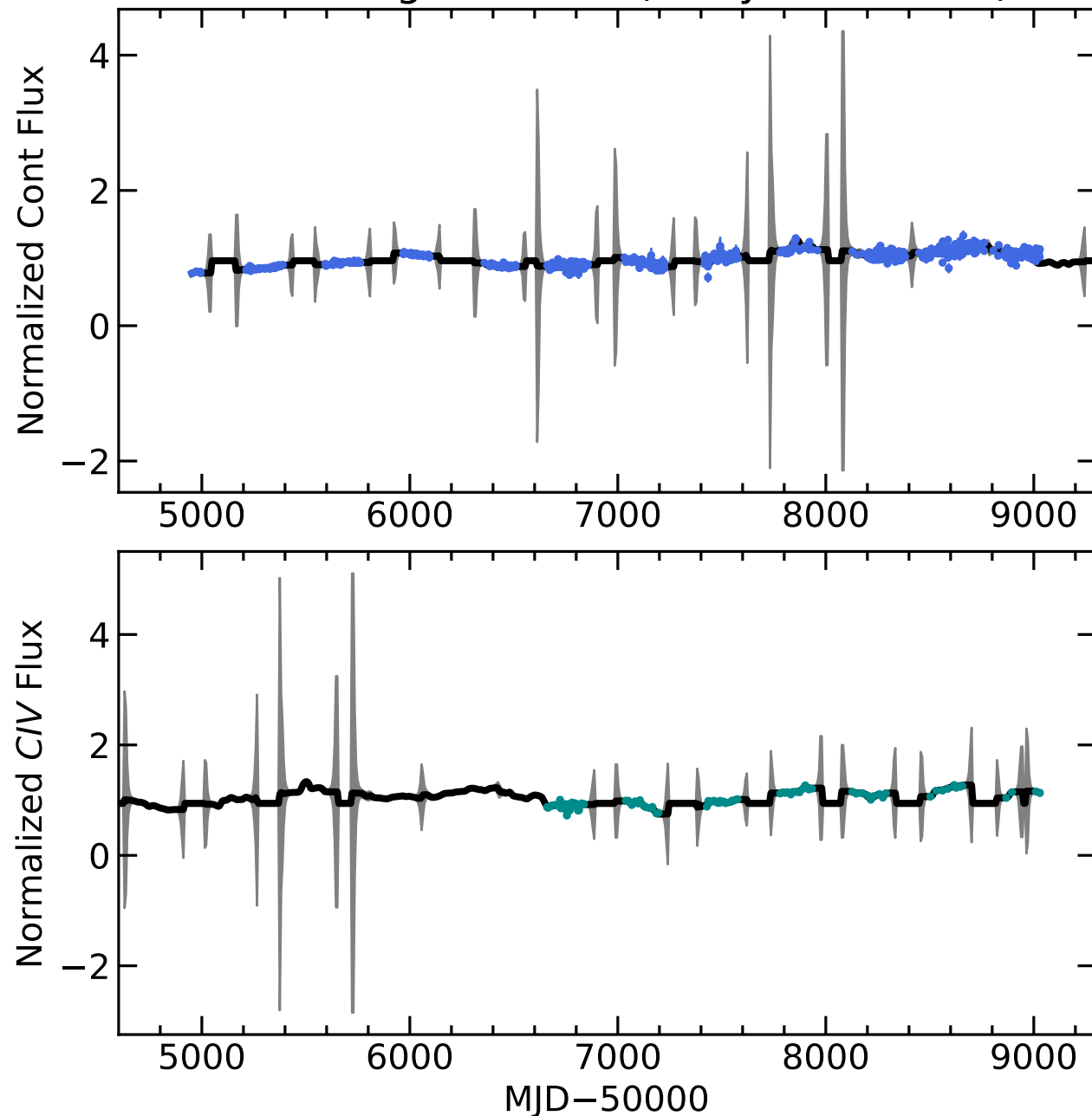
RM786 Light Curves (w/ PyROA model)
