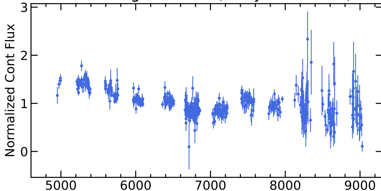
RM787 Light Curves (w/ PyROA model)
