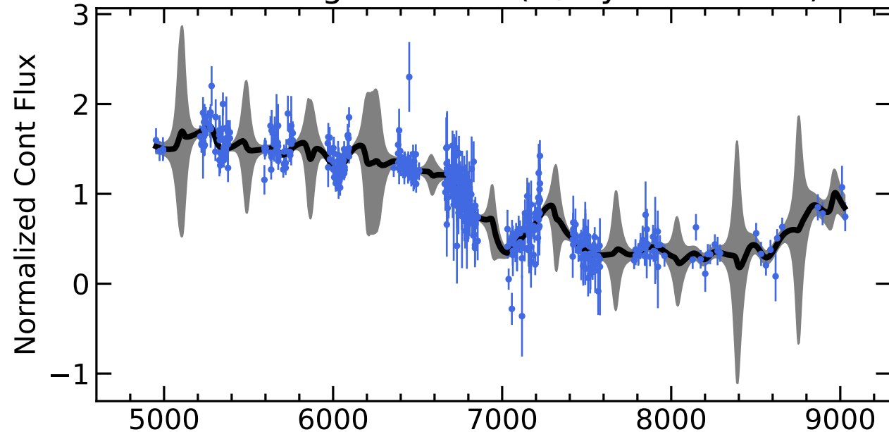
RM788 Light Curves (w/ PyROA model)
