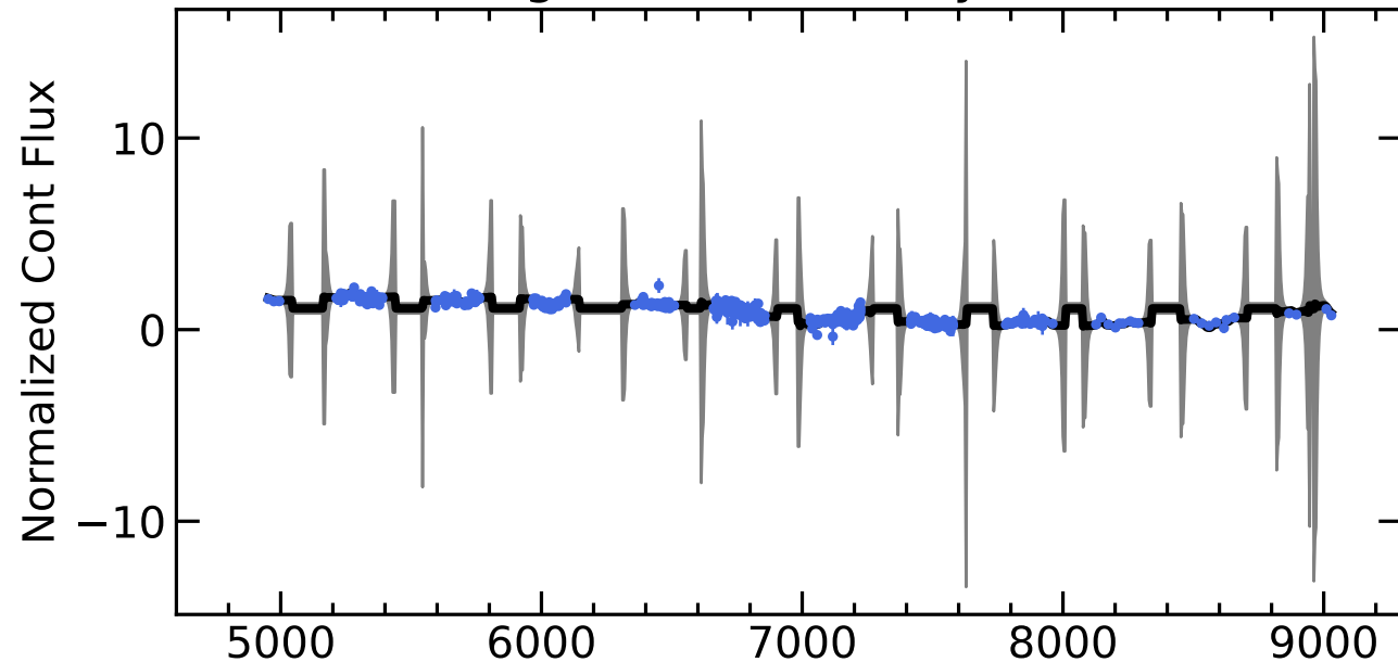
RM788 Light Curves (w/ PyROA model)
