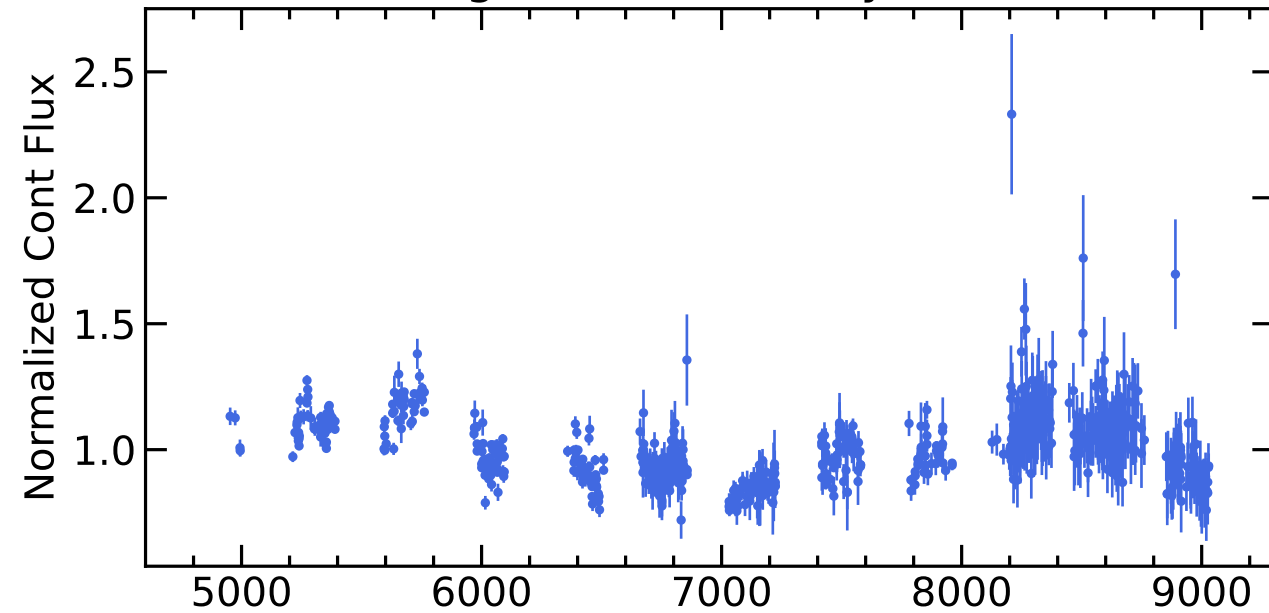
RM789 Light Curves (w/ PyROA model)
