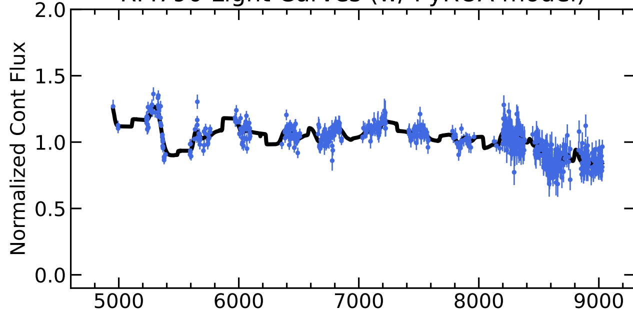
RM790 Light Curves (w/ PyROA model)
